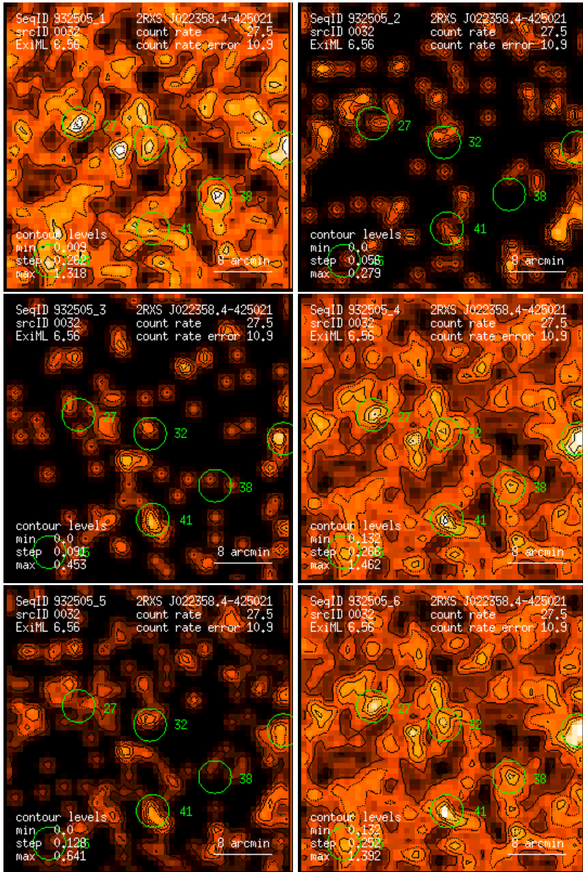
Figure 32: RASS 932505: detection 0032: band rate images, Gaussian filter: (1) PSPC channels 11 – 41, (2) 52 – 90, (3) 91 – 201, (4) 11 – 235, (5) 52 – 201, (6) 11 – 201. Broad band rates in counts/ks. Band rate contour levels in counts/ks/arcmin 2 .
