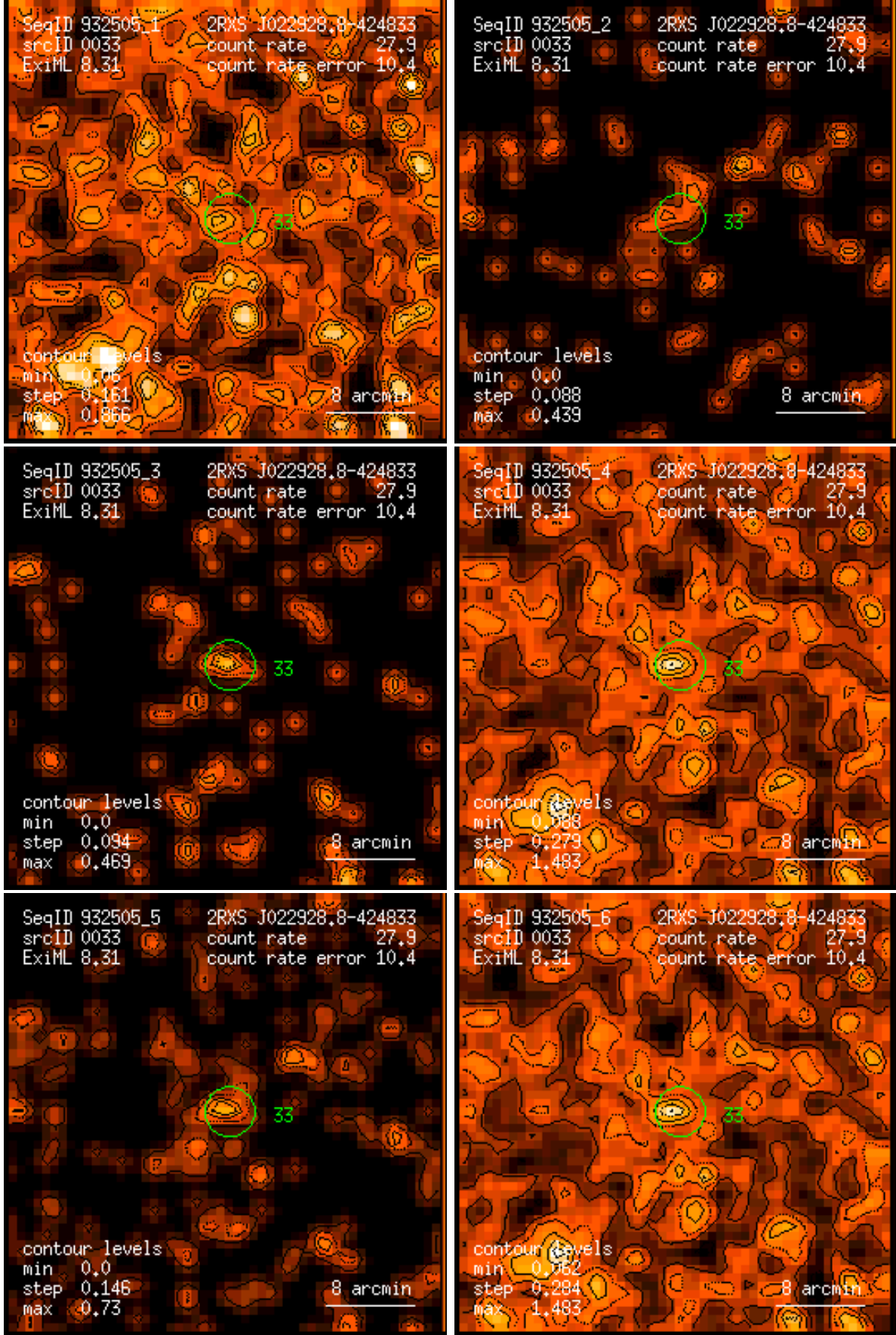
Figure 33: RASS 932505: detection 0033: band rate images, Gaussian filter: (1) PSPC channels 11 – 41, (2) 52 – 90, (3) 91 – 201, (4) 11 – 235, (5) 52 – 201, (6) 11 – 201. Broad band rates in counts/ks. Band rate contour levels in counts/ks/arcmin 2 .
