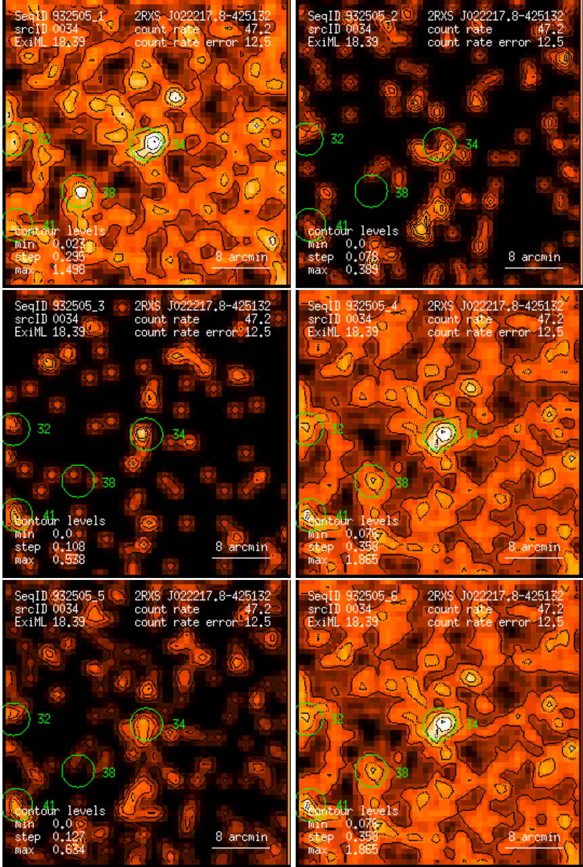
Figure 34: RASS 932505: detection 0034: band rate images, Gaussian filter: (1) PSPC channels 11 – 41, (2) 52 – 90, (3) 91 – 201, (4) 11 – 235, (5) 52 – 201, (6) 11 – 201. Broad band rates in counts/ks. Band rate contour levels in counts/ks/arcmin 2 .
