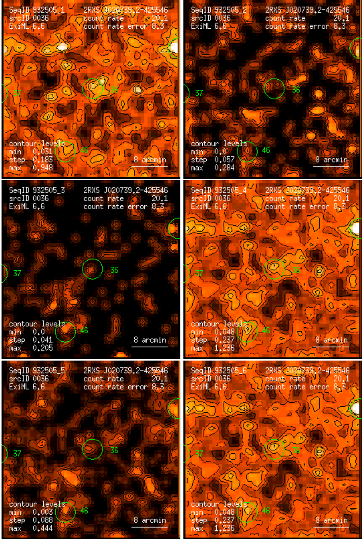
Figure 36: RASS 932505: detection 0036: band rate images, Gaussian filter: (1) PSPC channels 11 – 41, (2) 52 – 90, (3) 91 – 201, (4) 11 – 235, (5) 52 – 201, (6) 11 – 201. Broad band rates in counts/ks. Band rate contour levels in counts/ks/arcmin 2 .
