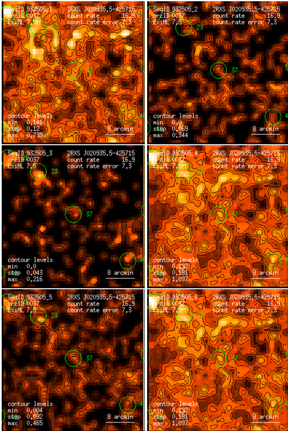
Figure 37: RASS 932505: detection 0037: band rate images, Gaussian filter: (1) PSPC channels 11 – 41, (2) 52 – 90, (3) 91 – 201, (4) 11 – 235, (5) 52 – 201, (6) 11 – 201. Broad band rates in counts/ks. Band rate contour levels in counts/ks/arcmin 2 .
