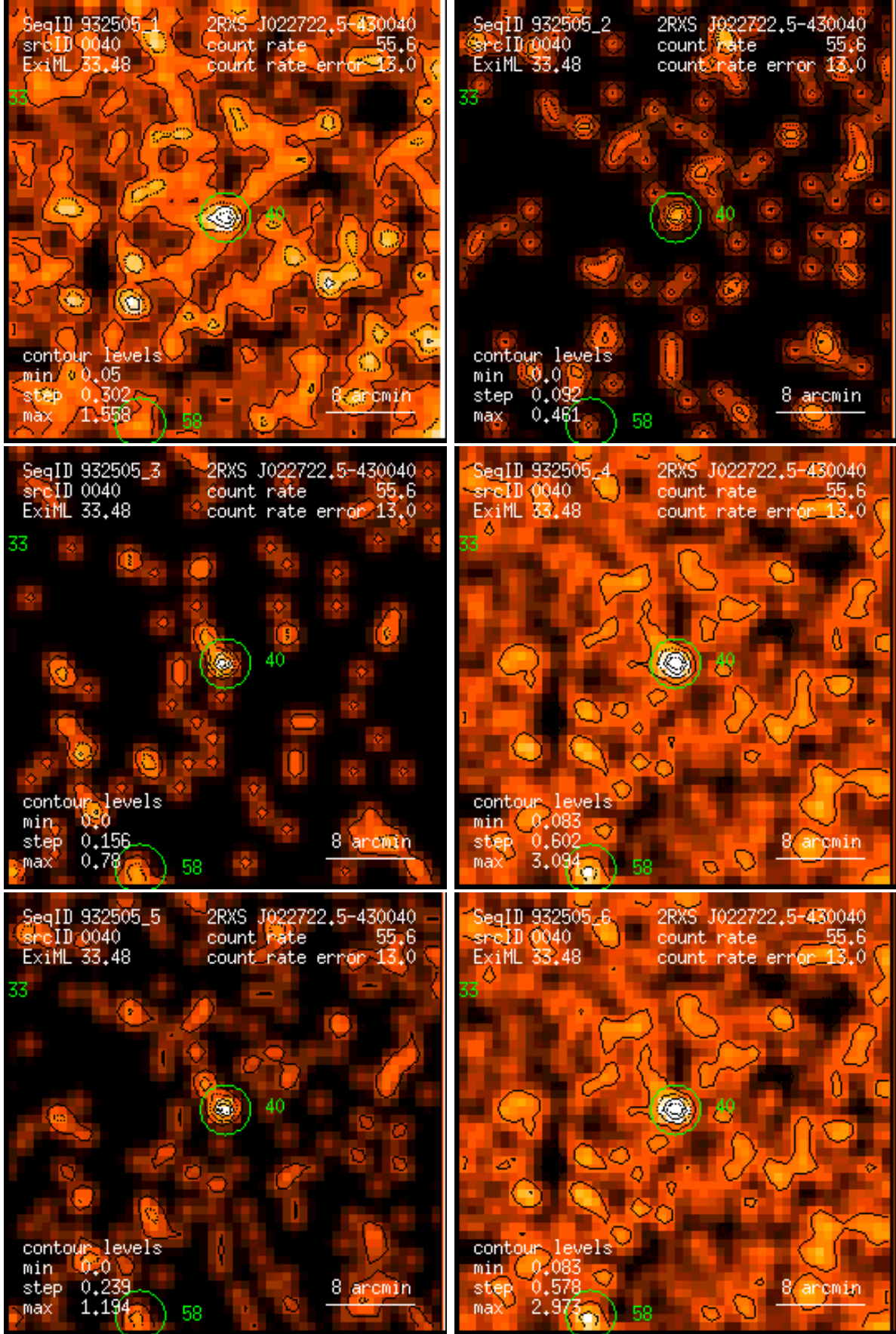
Figure 40: RASS 932505: detection 0040: band rate images, Gaussian filter: (1) PSPC channels 11 – 41, (2) 52 – 90, (3) 91 – 201, (4) 11 – 235, (5) 52 – 201, (6) 11 – 201. Broad band rates in counts/ks. Band rate contour levels in counts/ks/arcmin 2 .
