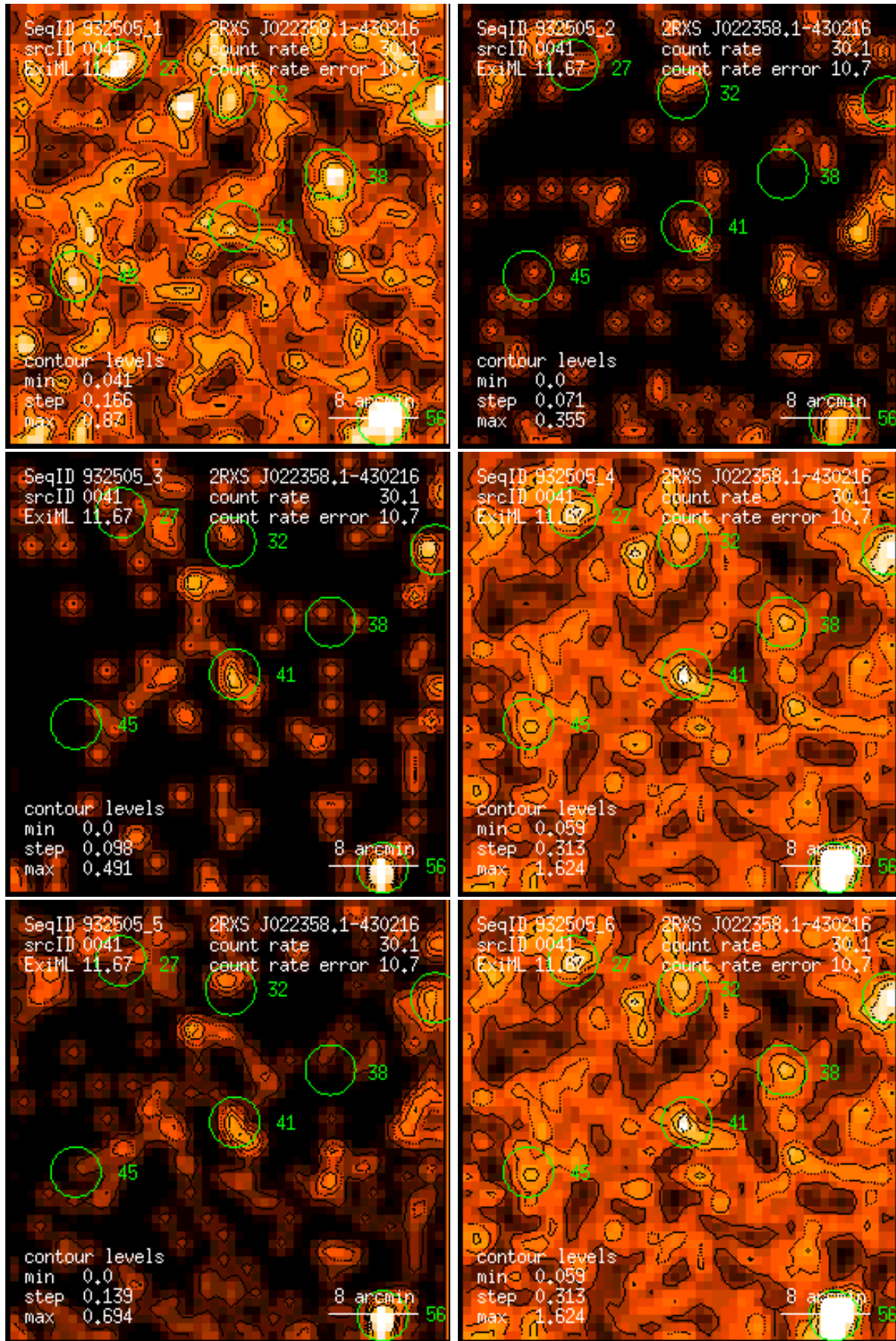
Figure 41: RASS 932505: detection 0041: band rate images, Gaussian filter: (1) PSPC channels 11 – 41, (2) 52 – 90, (3) 91 – 201, (4) 11 – 235, (5) 52 – 201, (6) 11 – 201. Broad band rates in counts/ks. Band rate contour levels in counts/ks/arcmin 2 .
