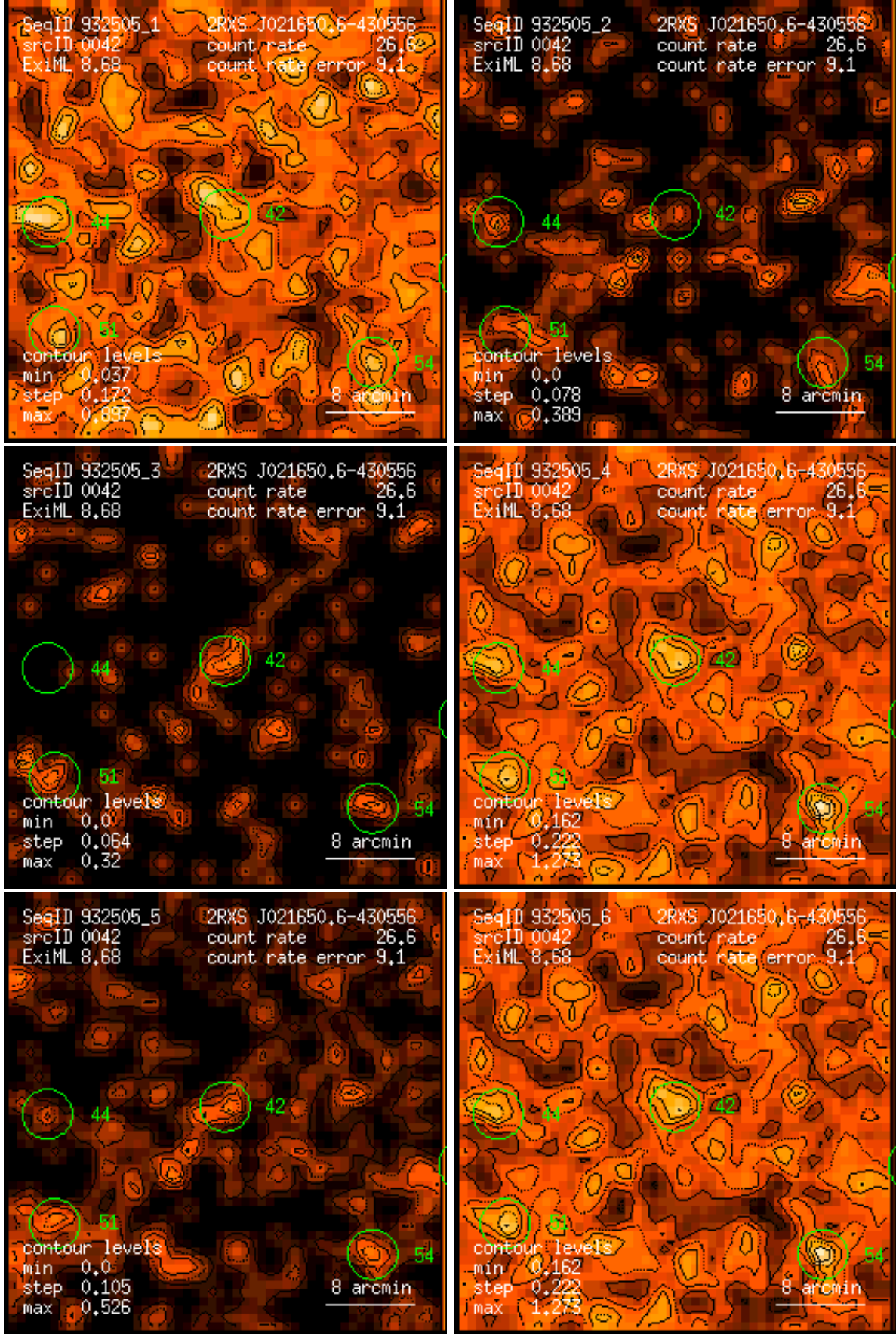
Figure 42: RASS 932505: detection 0042: band rate images, Gaussian filter: (1) PSPC channels 11 – 41, (2) 52 – 90, (3) 91 – 201, (4) 11 – 235, (5) 52 – 201, (6) 11 – 201. Broad band rates in counts/ks. Band rate contour levels in counts/ks/arcmin 2 .
