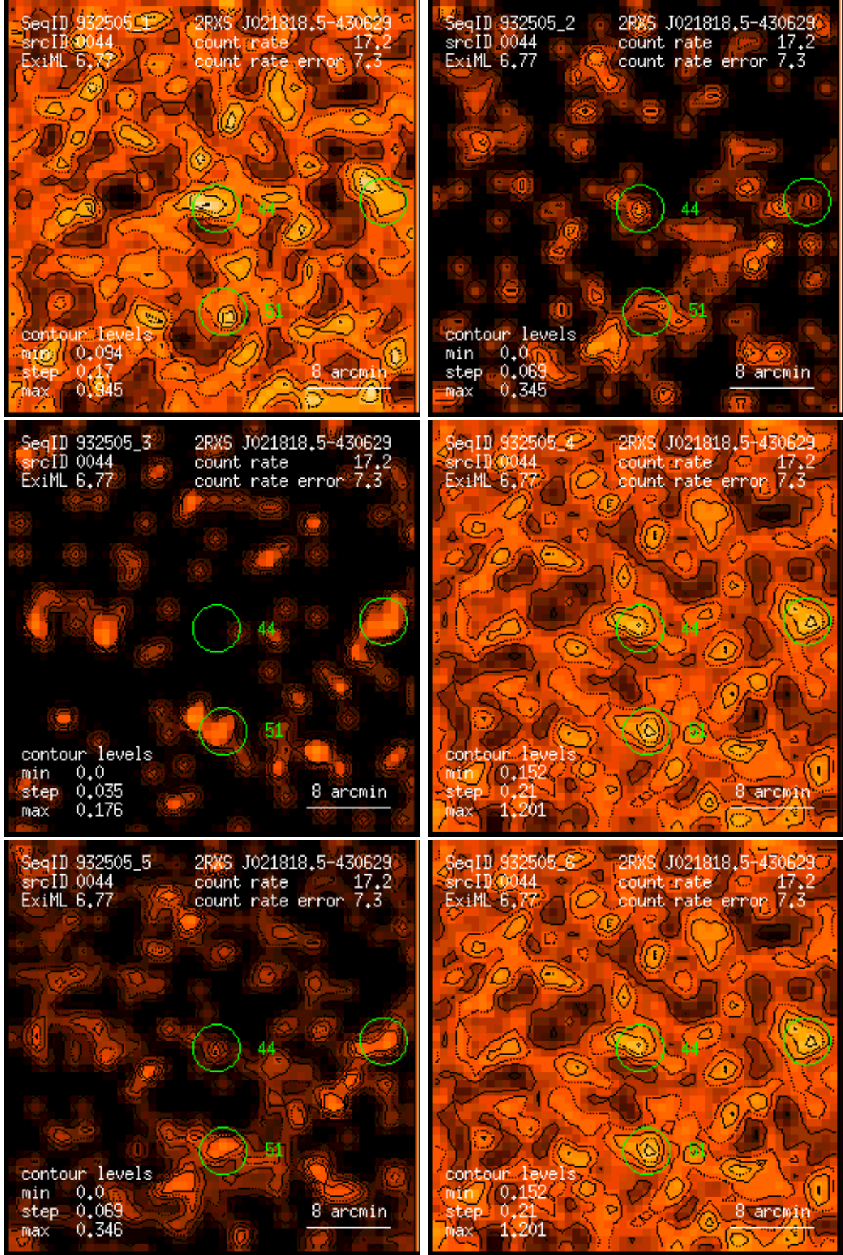
Figure 44: RASS 932505: detection 0044: band rate images, Gaussian filter: (1) PSPC channels 11 – 41, (2) 52 – 90, (3) 91 – 201, (4) 11 – 235, (5) 52 – 201, (6) 11 – 201. Broad band rates in counts/ks. Band rate contour levels in counts/ks/arcmin 2 .
