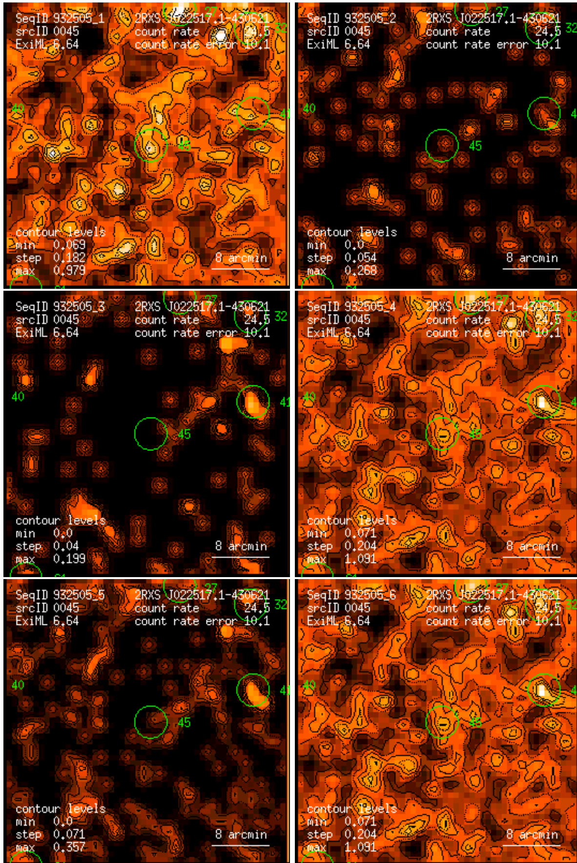
Figure 45: RASS 932505: detection 0045: band rate images, Gaussian filter: (1) PSPC channels 11 – 41, (2) 52 – 90, (3) 91 – 201, (4) 11 – 235, (5) 52 – 201, (6) 11 – 201. Broad band rates in counts/ks. Band rate contour levels in counts/ks/arcmin 2 .
