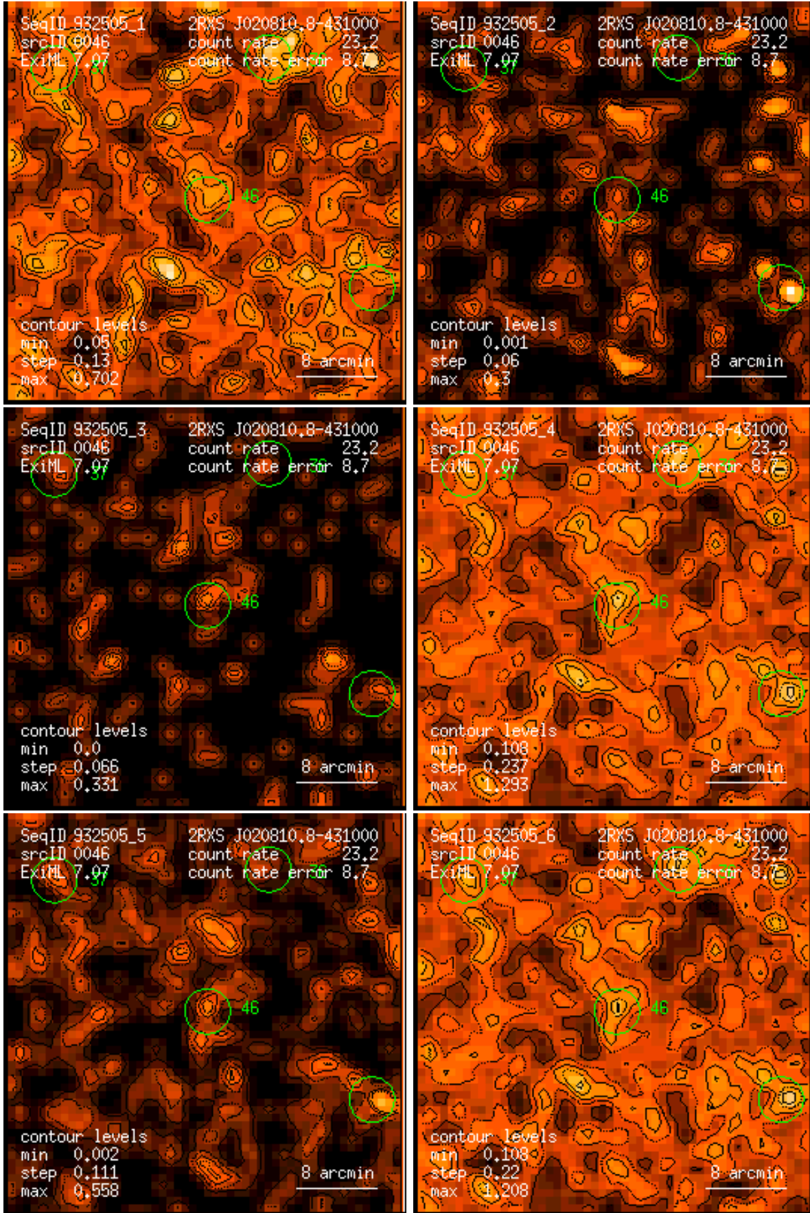
Figure 46: RASS 932505: detection 0046: band rate images, Gaussian filter: (1) PSPC channels 11 – 41, (2) 52 – 90, (3) 91 – 201, (4) 11 – 235, (5) 52 – 201, (6) 11 – 201. Broad band rates in counts/ks. Band rate contour levels in counts/ks/arcmin 2 .
