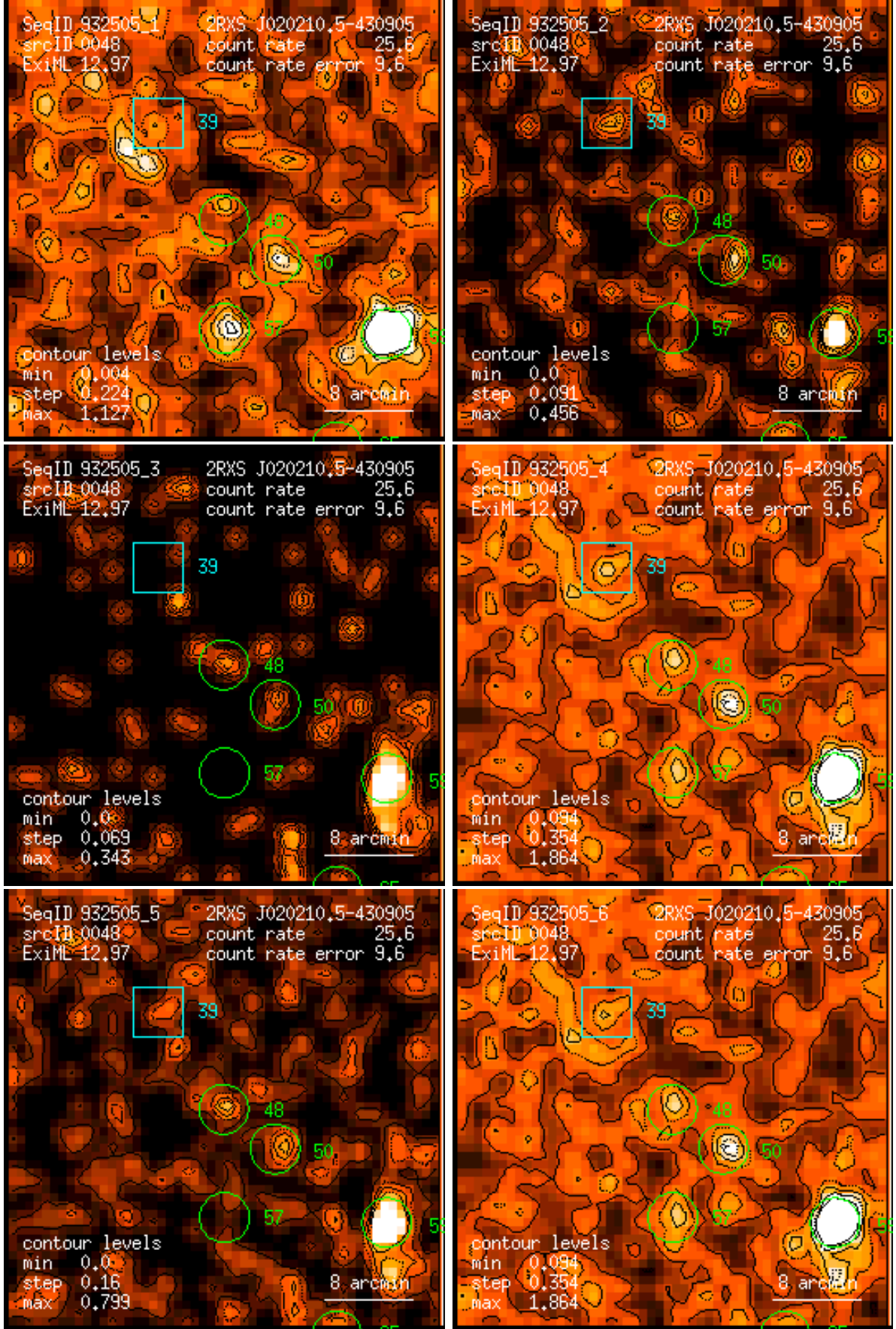
Figure 48: RASS 932505: detection 0048: band rate images, Gaussian filter: (1) PSPC channels 11 – 41, (2) 52 – 90, (3) 91 – 201, (4) 11 – 235, (5) 52 – 201, (6) 11 – 201. Broad band rates in counts/ks. Band rate contour levels in counts/ks/arcmin 2 .
