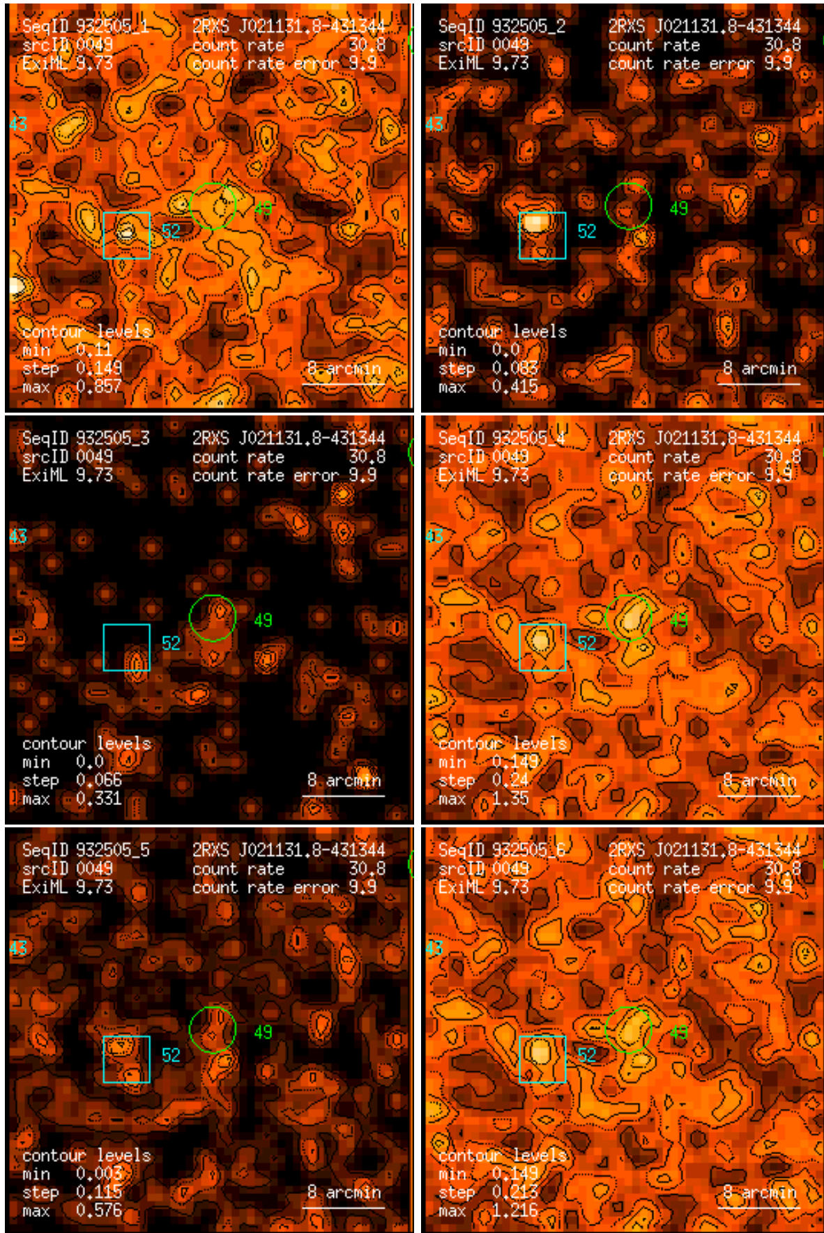
Figure 49: RASS 932505: detection 0049: band rate images, Gaussian filter: (1) PSPC channels 11 – 41, (2) 52 – 90, (3) 91 – 201, (4) 11 – 235, (5) 52 – 201, (6) 11 – 201. Broad band rates in counts/ks. Band rate contour levels in counts/ks/arcmin 2 .
