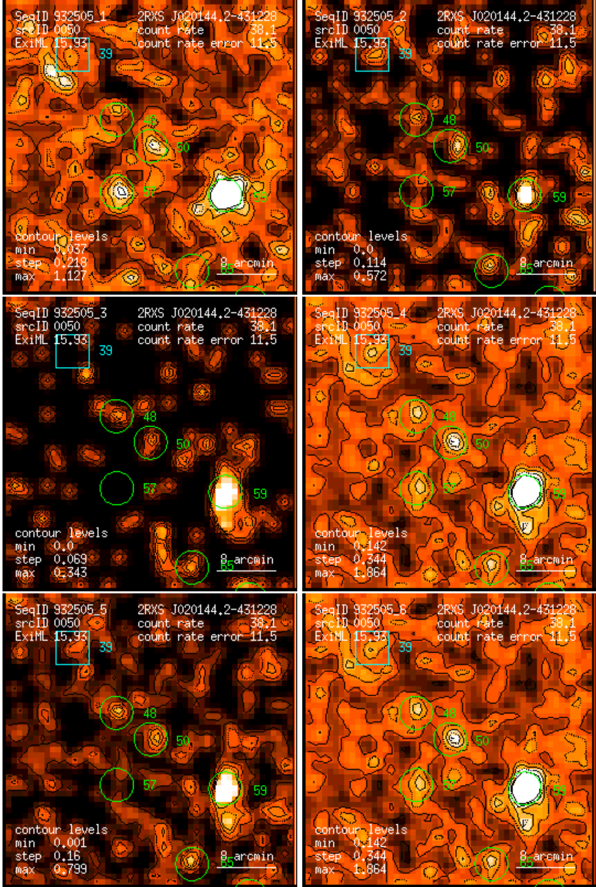
Figure 50: RASS 932505: detection 0050: band rate images, Gaussian filter: (1) PSPC channels 11 – 41, (2) 52 – 90, (3) 91 – 201, (4) 11 – 235, (5) 52 – 201, (6) 11 – 201. Broad band rates in counts/ks. Band rate contour levels in counts/ks/arcmin 2 .
