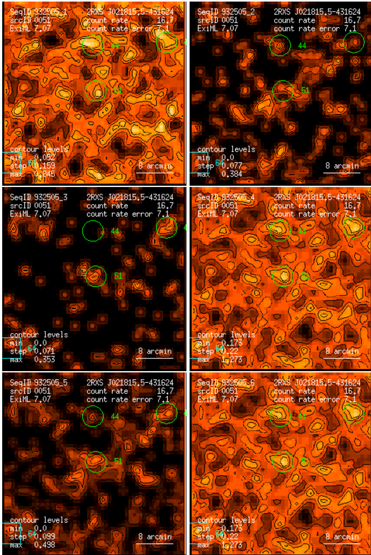
Figure 51: RASS 932505: detection 0051: band rate images, Gaussian filter: (1) PSPC channels 11 – 41, (2) 52 – 90, (3) 91 – 201, (4) 11 – 235, (5) 52 – 201, (6) 11 – 201. Broad band rates in counts/ks. Band rate contour levels in counts/ks/arcmin 2 .
