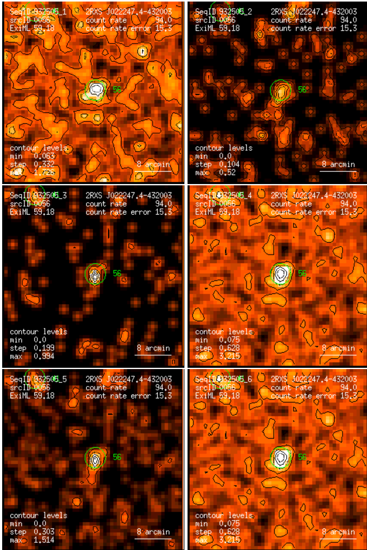
Figure 56: RASS 932505: detection 0056: band rate images, Gaussian filter: (1) PSPC channels 11 – 41, (2) 52 – 90, (3) 91 – 201, (4) 11 – 235, (5) 52 – 201, (6) 11 – 201. Broad band rates in counts/ks. Band rate contour levels in counts/ks/arcmin 2 .
