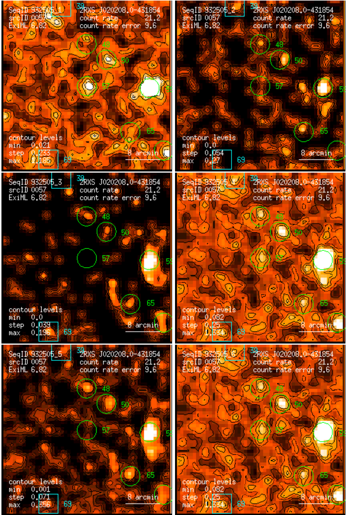
Figure 57: RASS 932505: detection 0057: band rate images, Gaussian filter: (1) PSPC channels 11 – 41, (2) 52 – 90, (3) 91 – 201, (4) 11 – 235, (5) 52 – 201, (6) 11 – 201. Broad band rates in counts/ks. Band rate contour levels in counts/ks/arcmin 2 .
