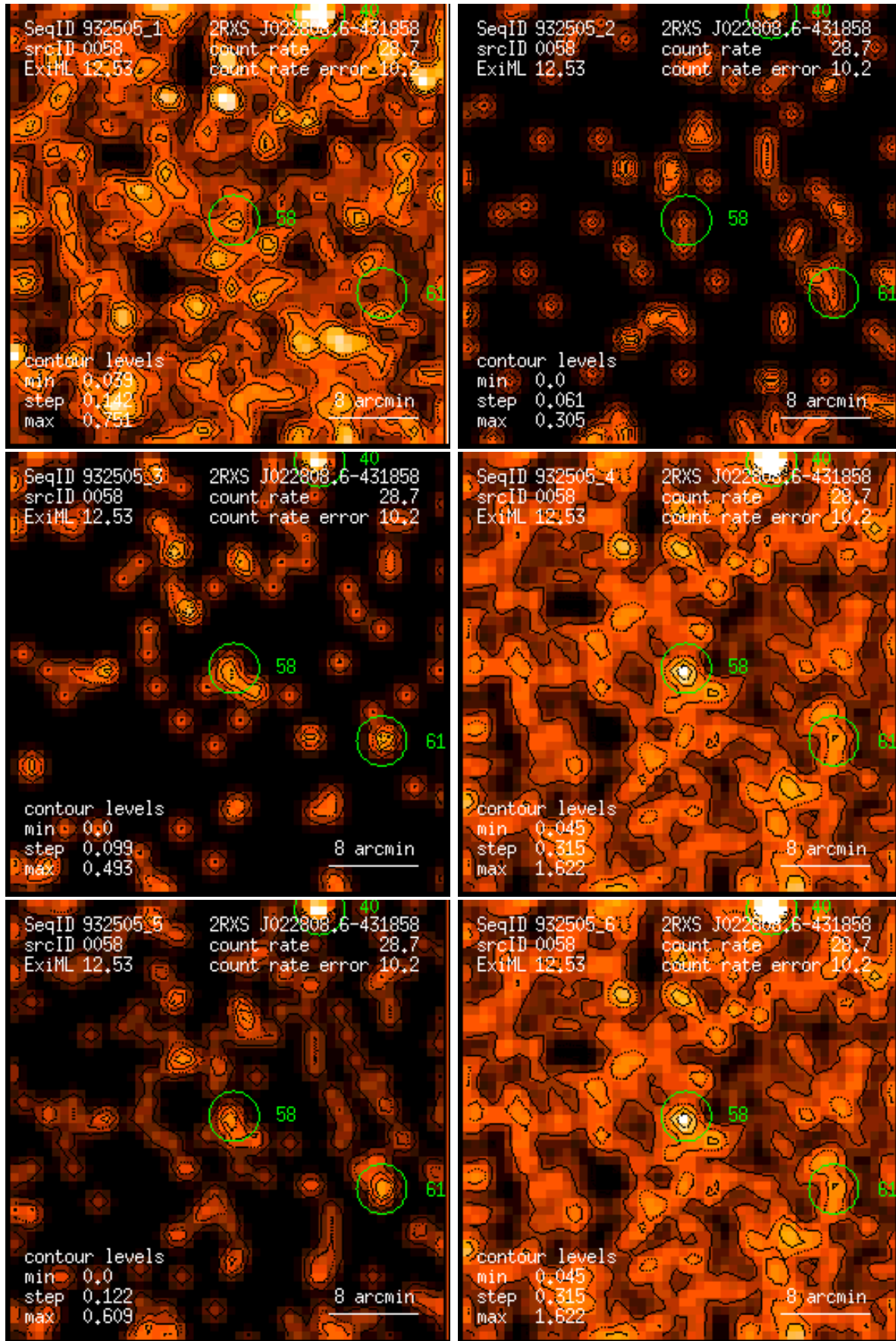
Figure 58: RASS 932505: detection 0058: band rate images, Gaussian filter: (1) PSPC channels 11 – 41, (2) 52 – 90, (3) 91 – 201, (4) 11 – 235, (5) 52 – 201, (6) 11 – 201. Broad band rates in counts/ks. Band rate contour levels in counts/ks/arcmin 2 .
