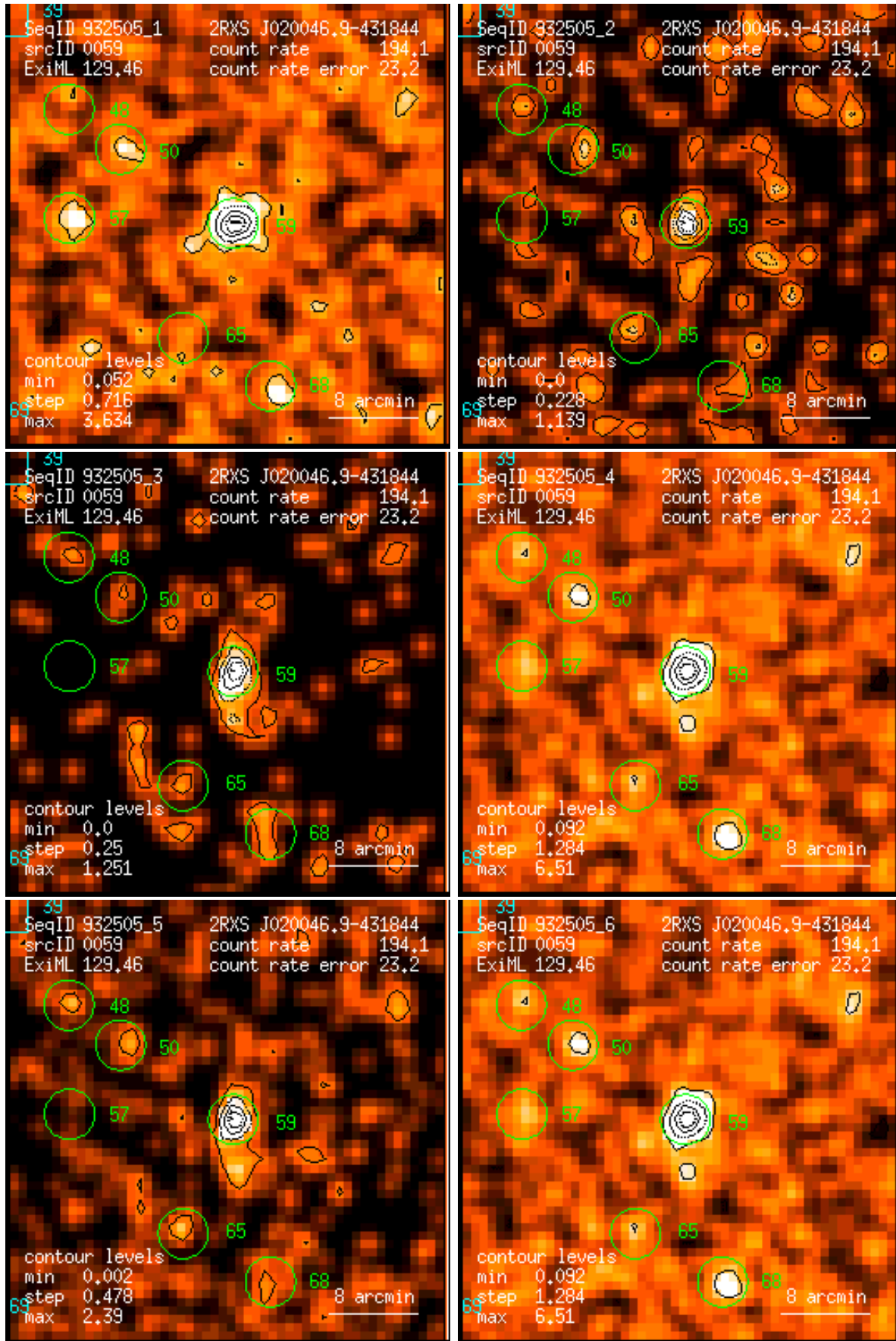
Figure 59: RASS 932505: detection 0059: band rate images, Gaussian filter: (1) PSPC channels 11 – 41, (2) 52 – 90, (3) 91 – 201, (4) 11 – 235, (5) 52 – 201, (6) 11 – 201. Broad band rates in counts/ks. Band rate contour levels in counts/ks/arcmin 2 .
