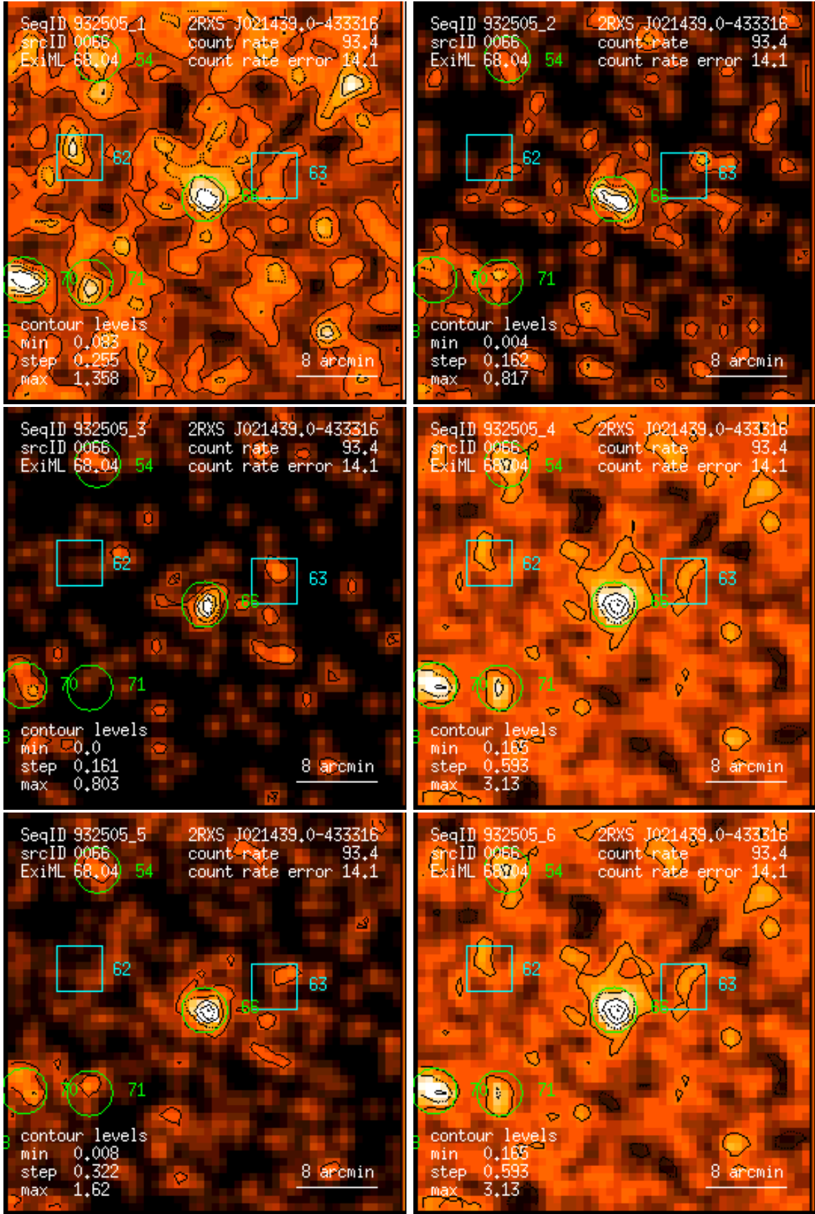
Figure 66: RASS 932505: detection 0066: band rate images, Gaussian filter: (1) PSPC channels 11 – 41, (2) 52 – 90, (3) 91 – 201, (4) 11 – 235, (5) 52 – 201, (6) 11 – 201. Broad band rates in counts/ks. Band rate contour levels in counts/ks/arcmin 2 .
