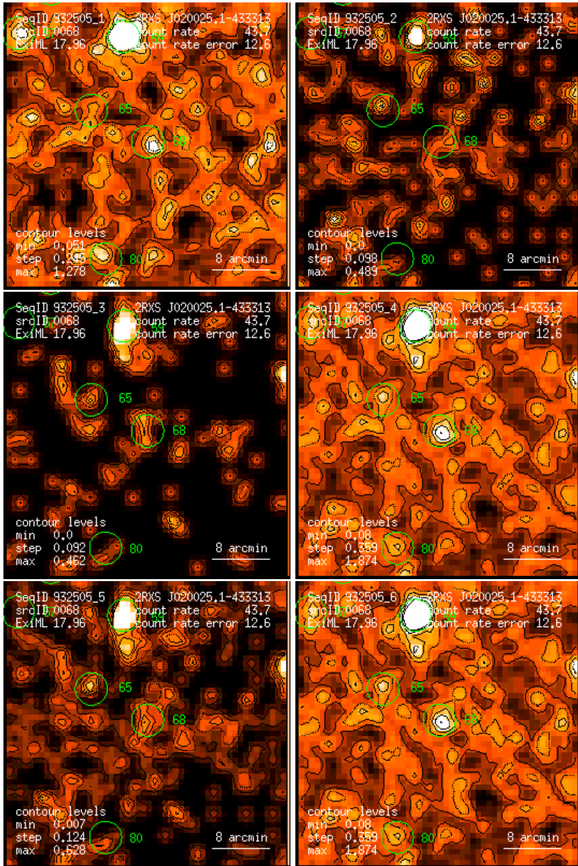
Figure 68: RASS 932505: detection 0068: band rate images, Gaussian filter: (1) PSPC channels 11 – 41, (2) 52 – 90, (3) 91 – 201, (4) 11 – 235, (5) 52 – 201, (6) 11 – 201. Broad band rates in counts/ks. Band rate contour levels in counts/ks/arcmin 2 .
