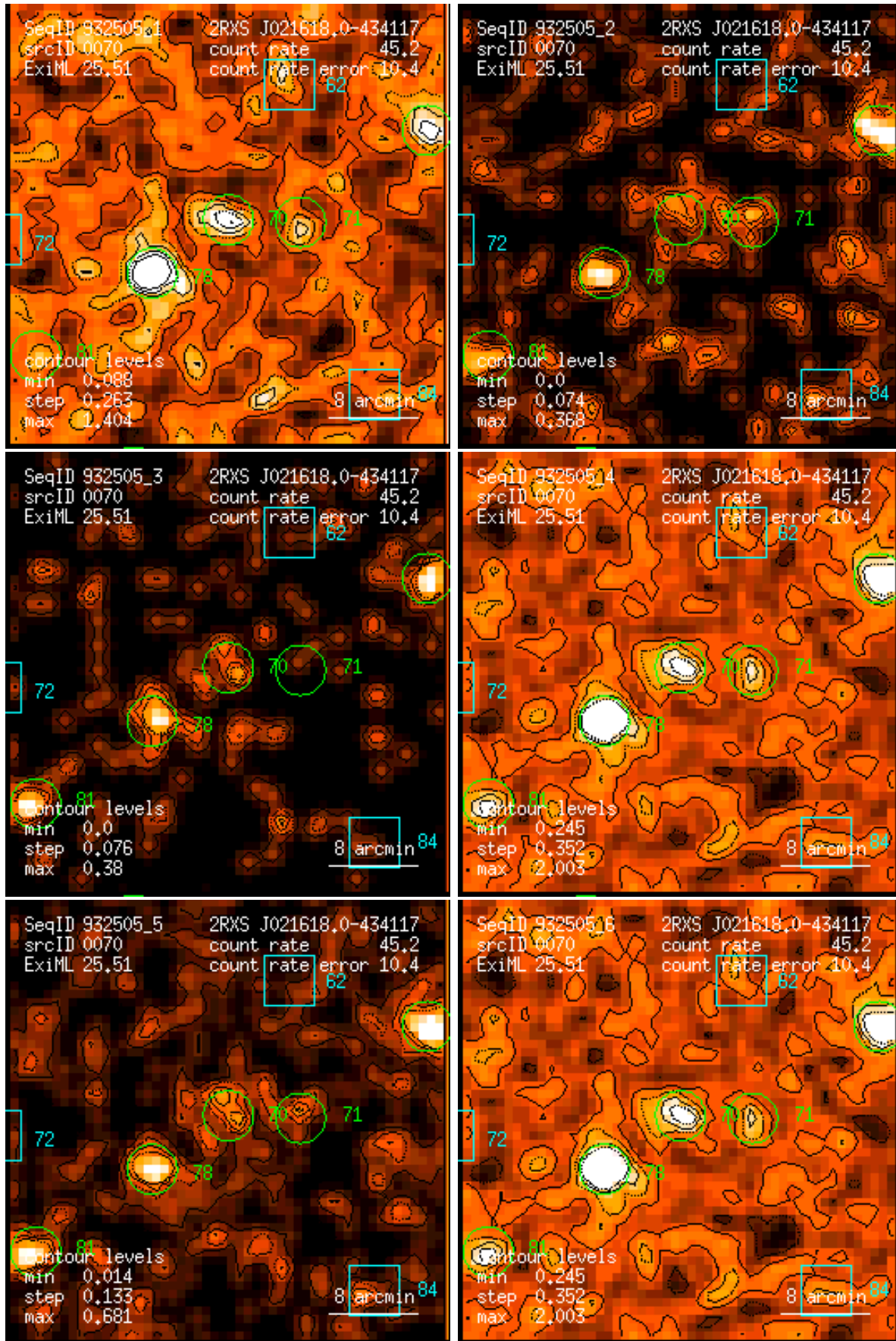
Figure 70: RASS 932505: detection 0070: band rate images, Gaussian filter: (1) PSPC channels 11 – 41, (2) 52 – 90, (3) 91 – 201, (4) 11 – 235, (5) 52 – 201, (6) 11 – 201. Broad band rates in counts/ks. Band rate contour levels in counts/ks/arcmin 2 .
