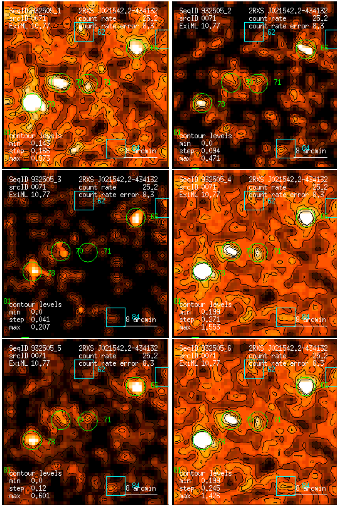
Figure 71: RASS 932505: detection 0071: band rate images, Gaussian filter: (1) PSPC channels 11 – 41, (2) 52 – 90, (3) 91 – 201, (4) 11 – 235, (5) 52 – 201, (6) 11 – 201. Broad band rates in counts/ks. Band rate contour levels in counts/ks/arcmin 2 .
