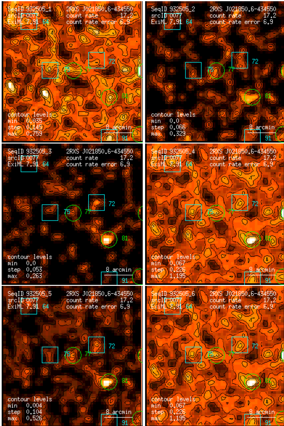
Figure 77: RASS 932505: detection 0077: band rate images, Gaussian filter: (1) PSPC channels 11 – 41, (2) 52 – 90, (3) 91 – 201, (4) 11 – 235, (5) 52 – 201, (6) 11 – 201. Broad band rates in counts/ks. Band rate contour levels in counts/ks/arcmin 2 .
