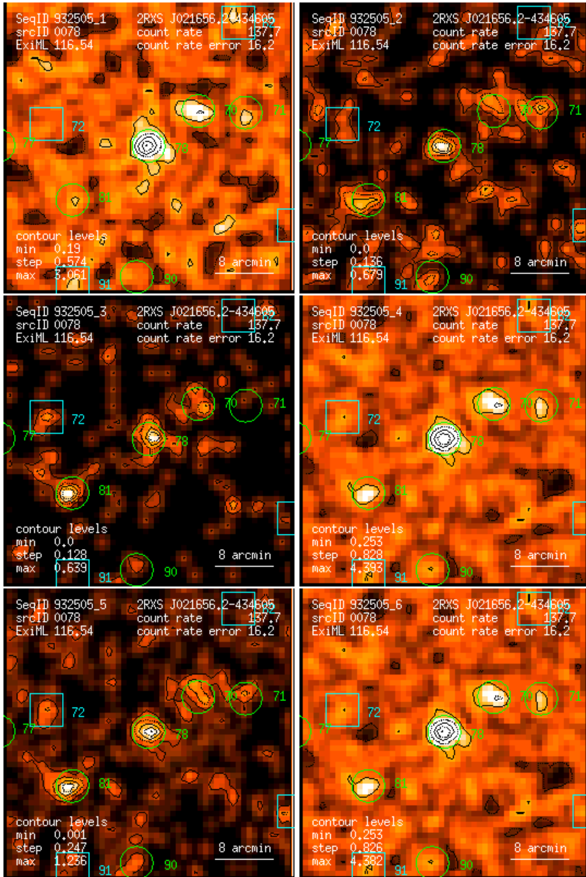
Figure 78: RASS 932505: detection 0078: band rate images, Gaussian filter: (1) PSPC channels 11 – 41, (2) 52 – 90, (3) 91 – 201, (4) 11 – 235, (5) 52 – 201, (6) 11 – 201. Broad band rates in counts/ks. Band rate contour levels in counts/ks/arcmin 2 .
