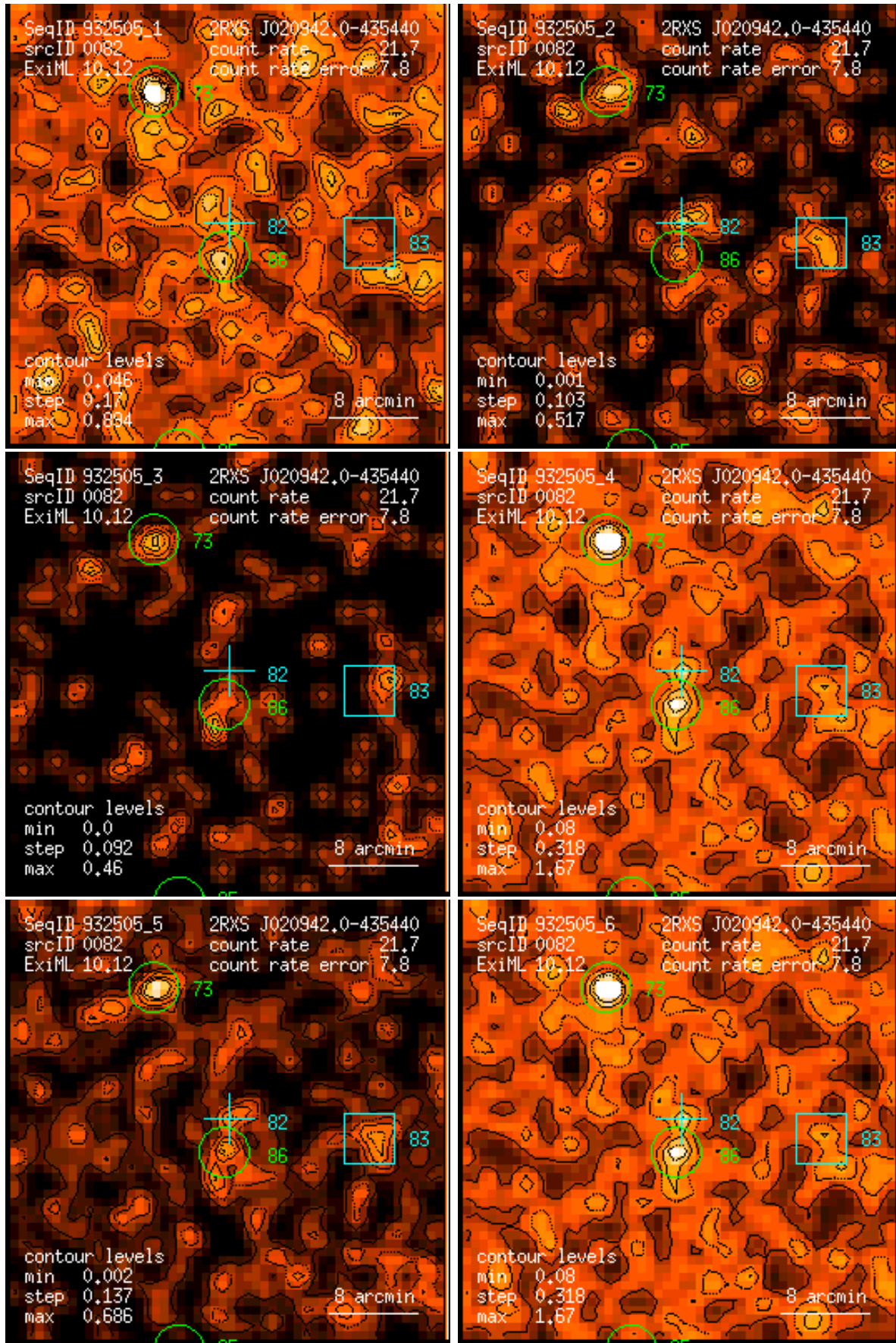
Figure 82: RASS 932505: detection 0082: band rate images, Gaussian filter: (1) PSPC channels 11 – 41, (2) 52 – 90, (3) 91 – 201, (4) 11 – 235, (5) 52 – 201, (6) 11 – 201. Broad band rates in counts/ks. Band rate contour levels in counts/ks/arcmin 2 .
