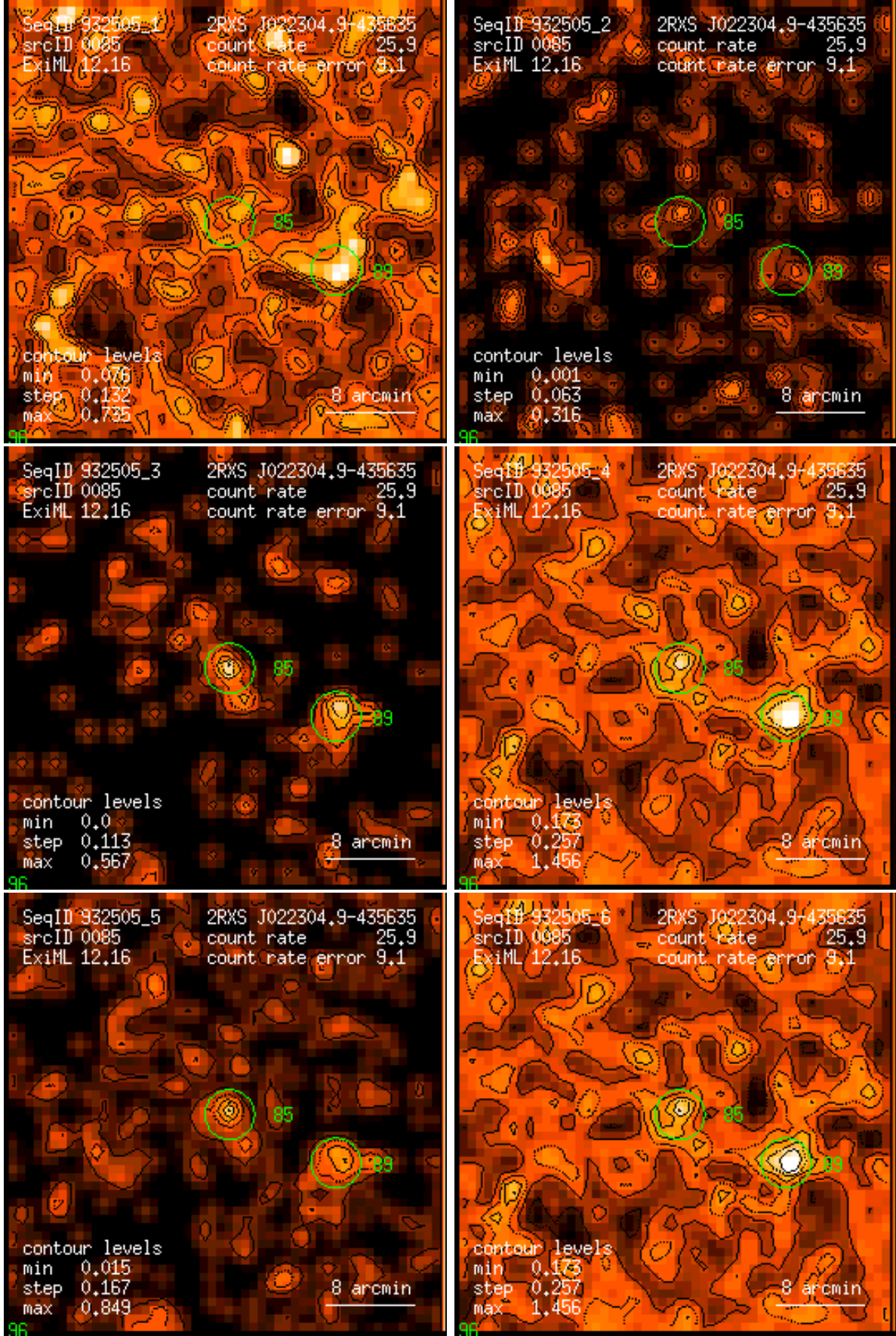
Figure 85: RASS 932505: detection 0085: band rate images, Gaussian filter: (1) PSPC channels 11 – 41, (2) 52 – 90, (3) 91 – 201, (4) 11 – 235, (5) 52 – 201, (6) 11 – 201. Broad band rates in counts/ks. Band rate contour levels in counts/ks/arcmin 2 .
