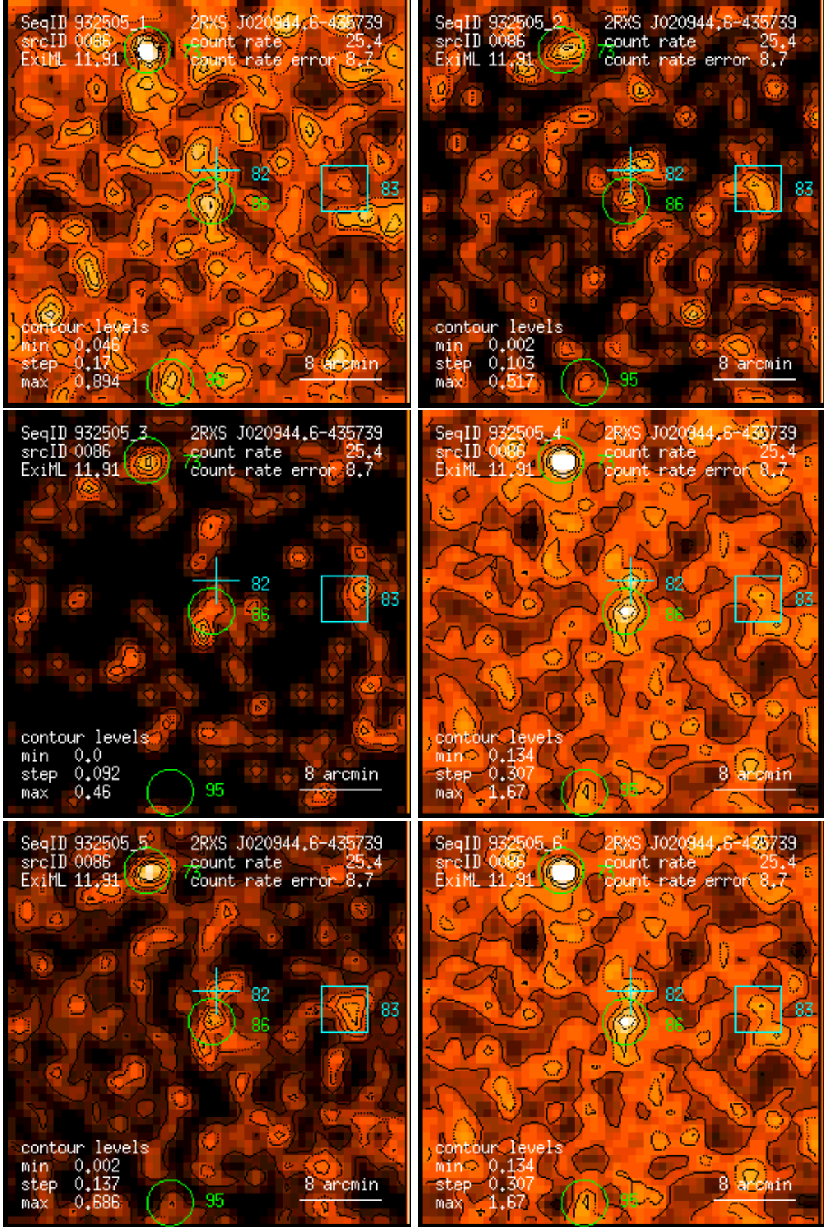
Figure 86: RASS 932505: detection 0086: band rate images, Gaussian filter: (1) PSPC channels 11 – 41, (2) 52 – 90, (3) 91 – 201, (4) 11 – 235, (5) 52 – 201, (6) 11 – 201. Broad band rates in counts/ks. Band rate contour levels in counts/ks/arcmin 2 .
