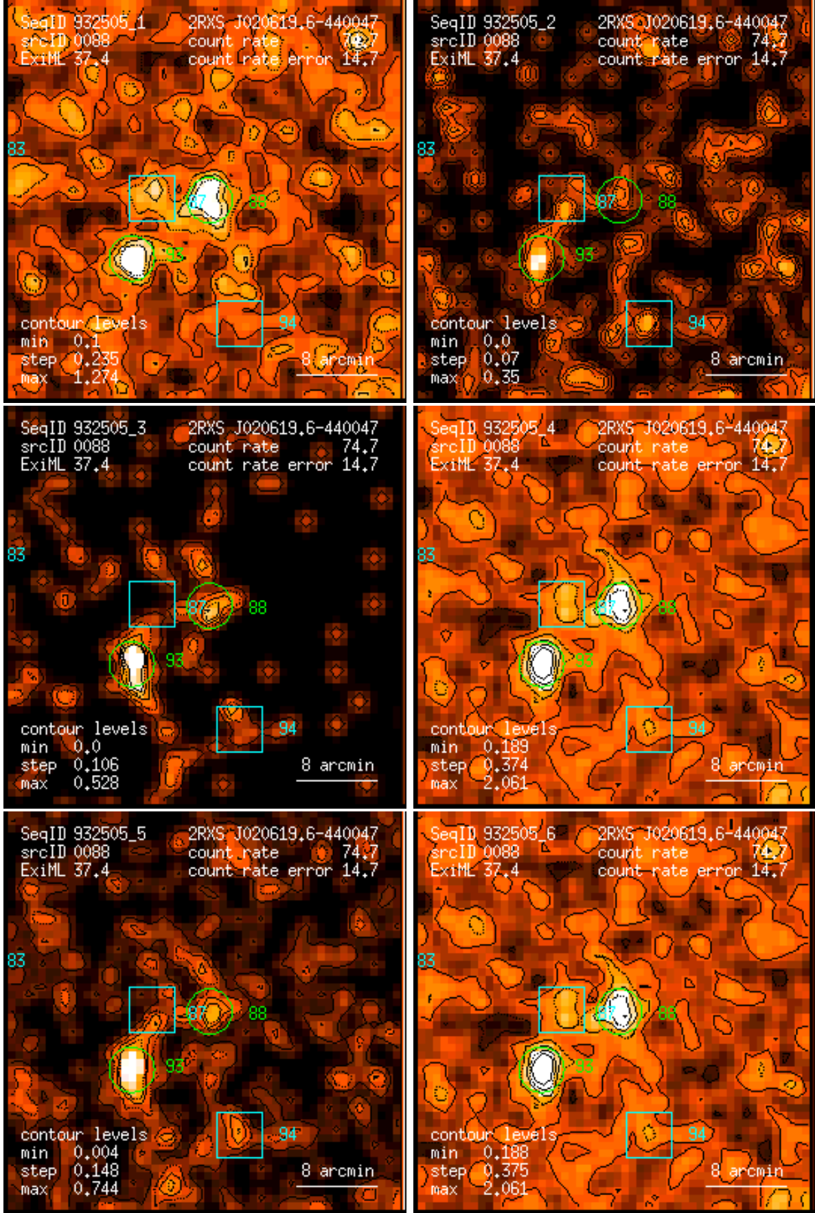
Figure 88: RASS 932505: detection 0088: band rate images, Gaussian filter: (1) PSPC channels 11 – 41, (2) 52 – 90, (3) 91 – 201, (4) 11 – 235, (5) 52 – 201, (6) 11 – 201. Broad band rates in counts/ks. Band rate contour levels in counts/ks/arcmin 2 .
