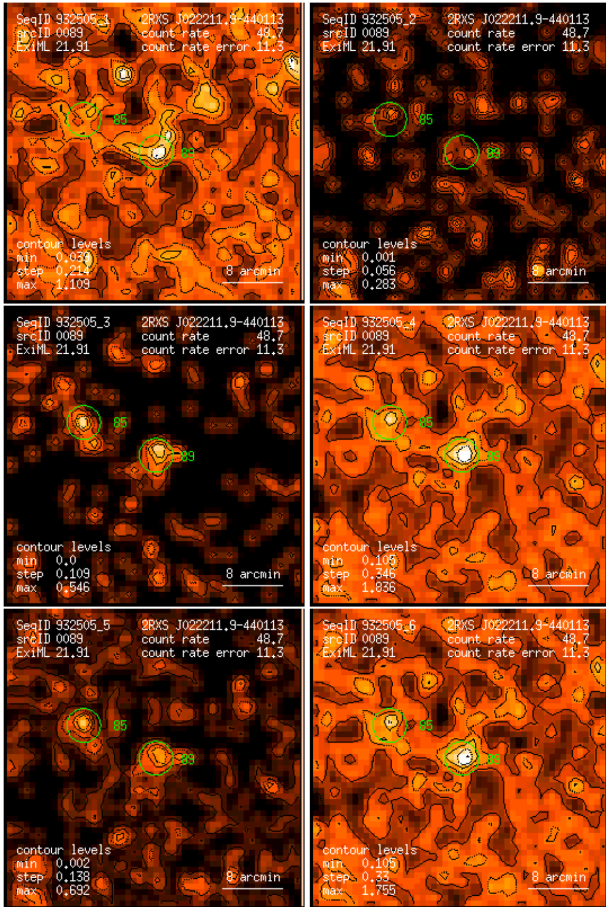
Figure 89: RASS 932505: detection 0089: band rate images, Gaussian filter: (1) PSPC channels 11 – 41, (2) 52 – 90, (3) 91 – 201, (4) 11 – 235, (5) 52 – 201, (6) 11 – 201. Broad band rates in counts/ks. Band rate contour levels in counts/ks/arcmin 2 .
