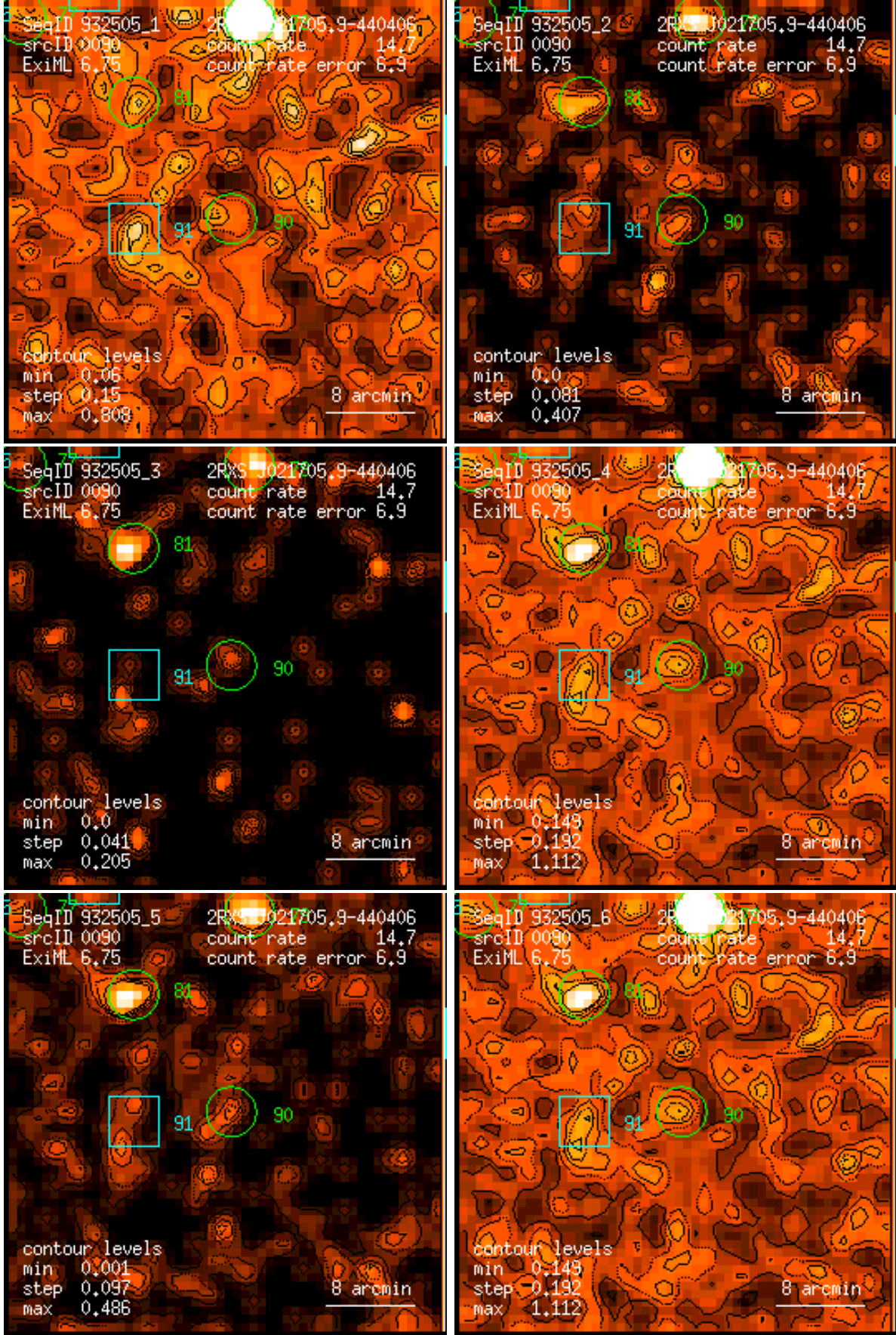
Figure 90: RASS 932505: detection 0090: band rate images, Gaussian filter: (1) PSPC channels 11 – 41, (2) 52 – 90, (3) 91 – 201, (4) 11 – 235, (5) 52 – 201, (6) 11 – 201. Broad band rates in counts/ks. Band rate contour levels in counts/ks/arcmin 2 .
