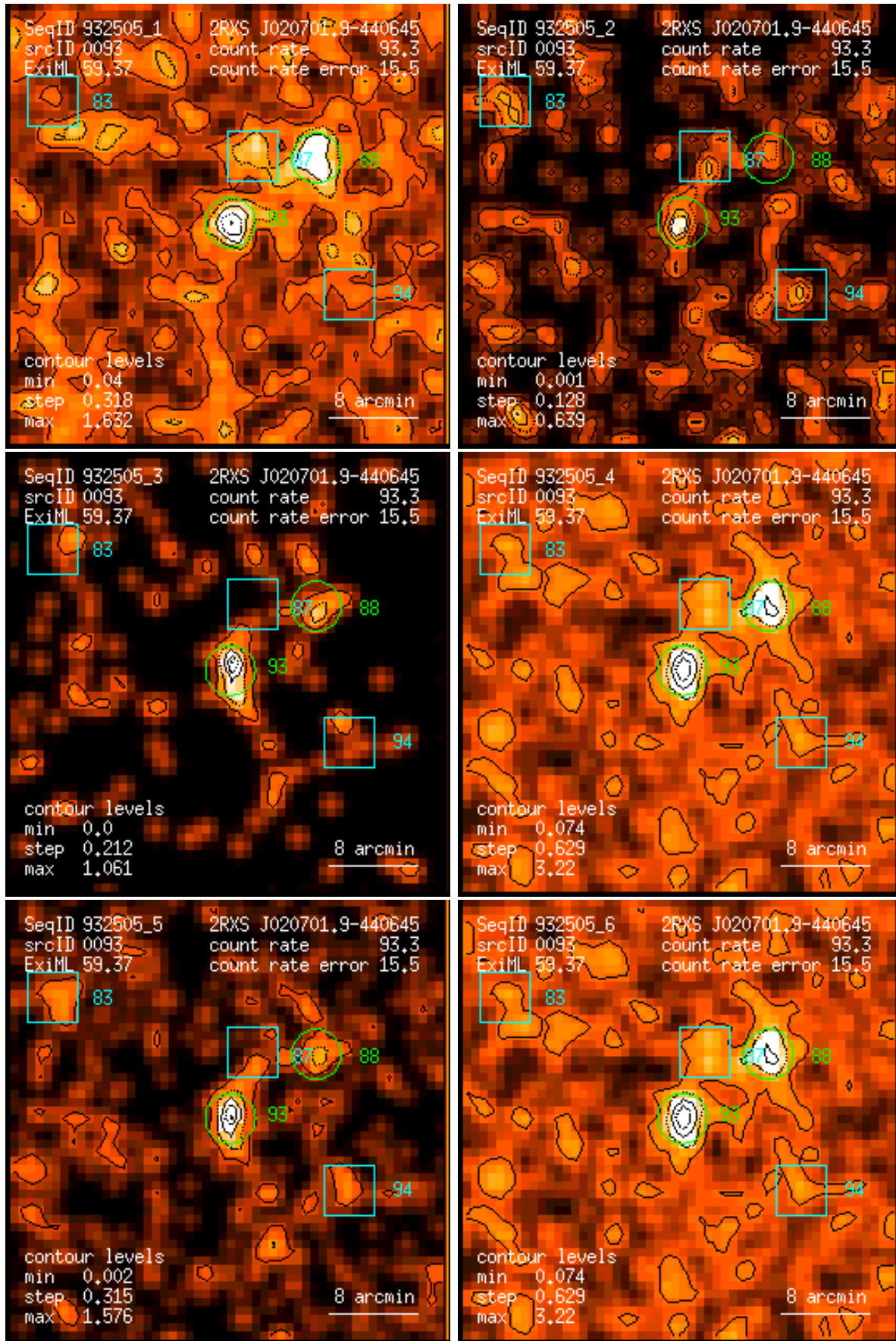
Figure 93: RASS 932505: detection 0093: band rate images, Gaussian filter: (1) PSPC channels 11 – 41, (2) 52 – 90, (3) 91 – 201, (4) 11 – 235, (5) 52 – 201, (6) 11 – 201. Broad band rates in counts/ks. Band rate contour levels in counts/ks/arcmin 2 .
