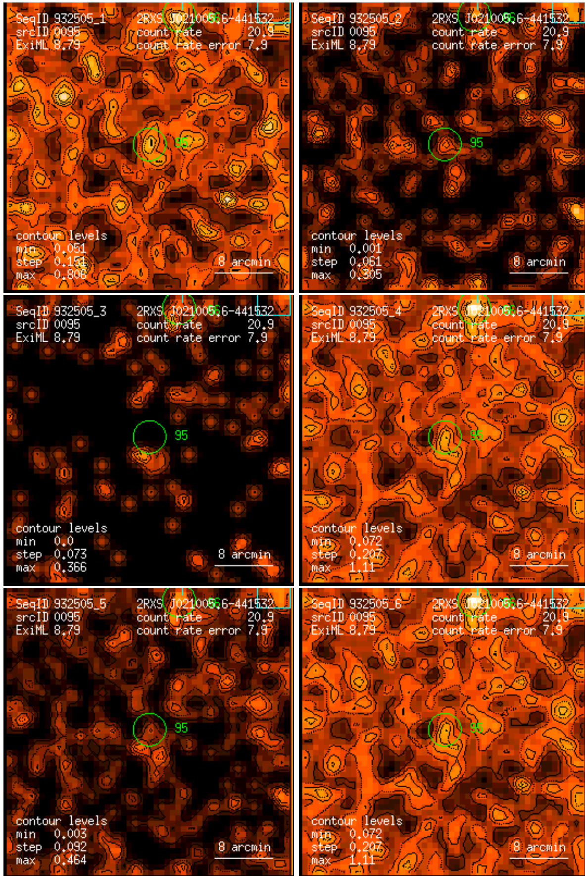
Figure 95: RASS 932505: detection 0095: band rate images, Gaussian filter: (1) PSPC channels 11 – 41, (2) 52 – 90, (3) 91 – 201, (4) 11 – 235, (5) 52 – 201, (6) 11 – 201. Broad band rates in counts/ks. Band rate contour levels in counts/ks/arcmin 2 .
