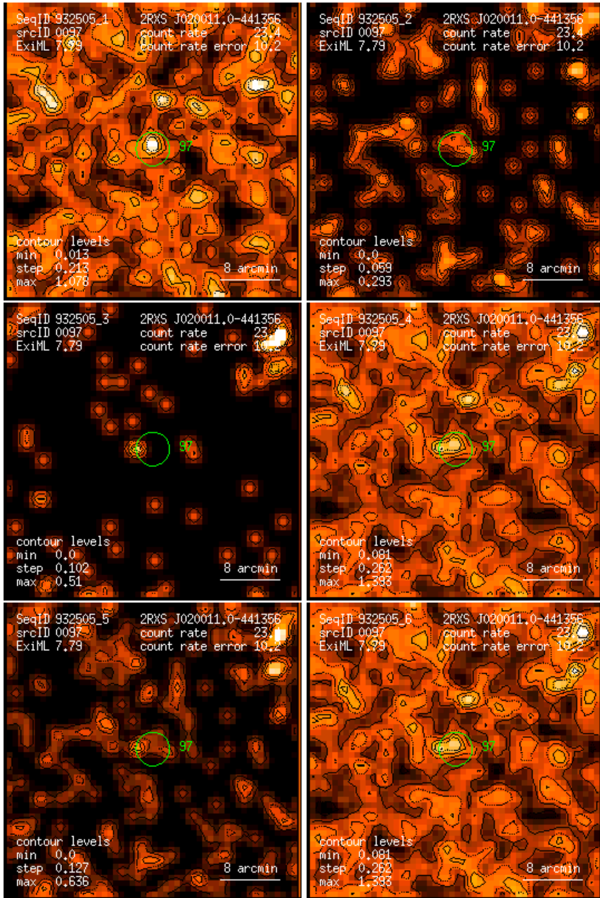
Figure 97: RASS 932505: detection 0097: band rate images, Gaussian filter: (1) PSPC channels 11 – 41, (2) 52 – 90, (3) 91 – 201, (4) 11 – 235, (5) 52 – 201, (6) 11 – 201. Broad band rates in counts/ks. Band rate contour levels in counts/ks/arcmin 2 .
