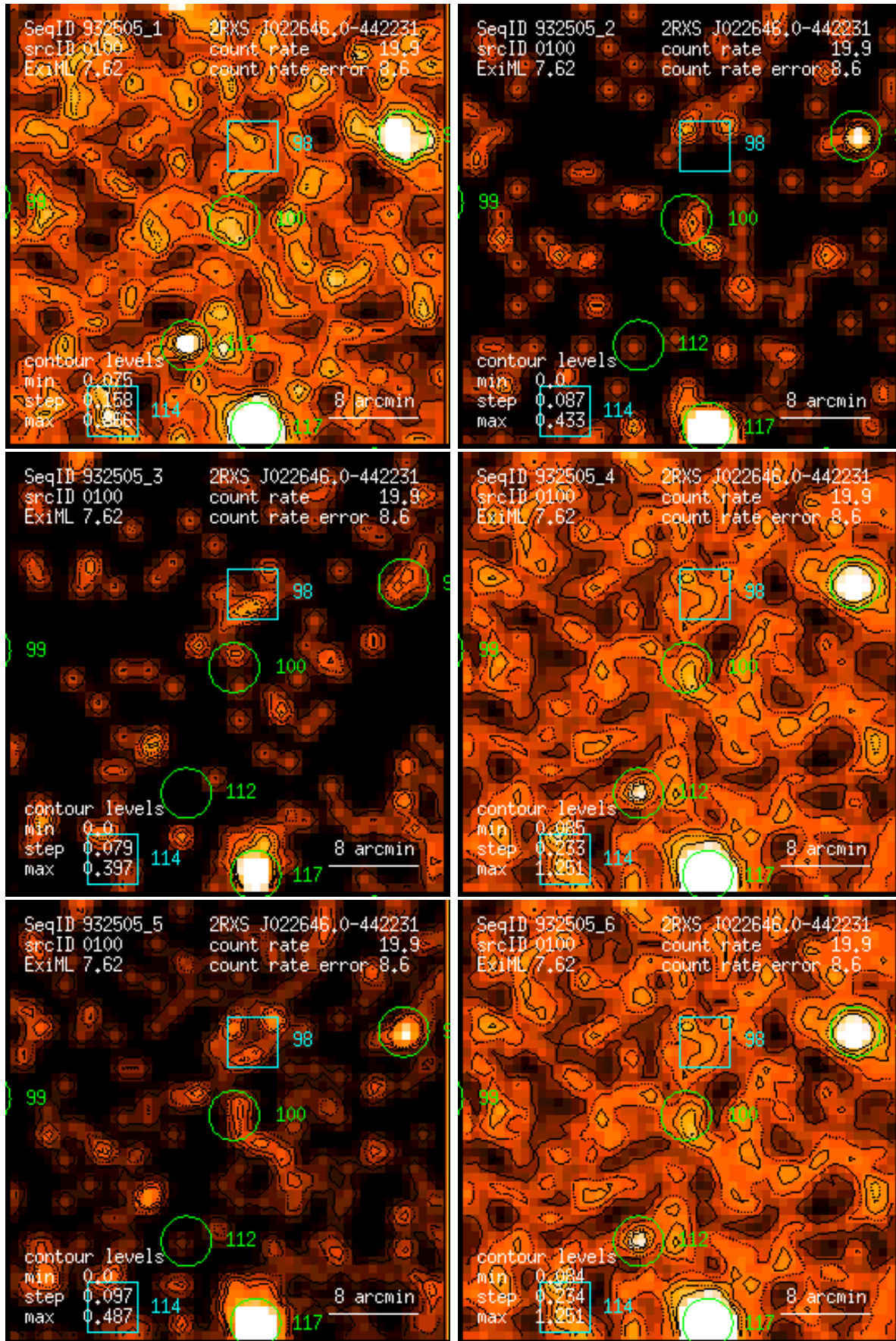
Figure 100: RASS 932505: detection 0100: band rate images, Gaussian filter: (1) PSPC channels 11 – 41, (2) 52 – 90, (3) 91 – 201, (4) 11 – 235, (5) 52 – 201, (6) 11 – 201. Broad band rates in counts/ks. Band rate contour levels in counts/ks/arcmin 2 .
