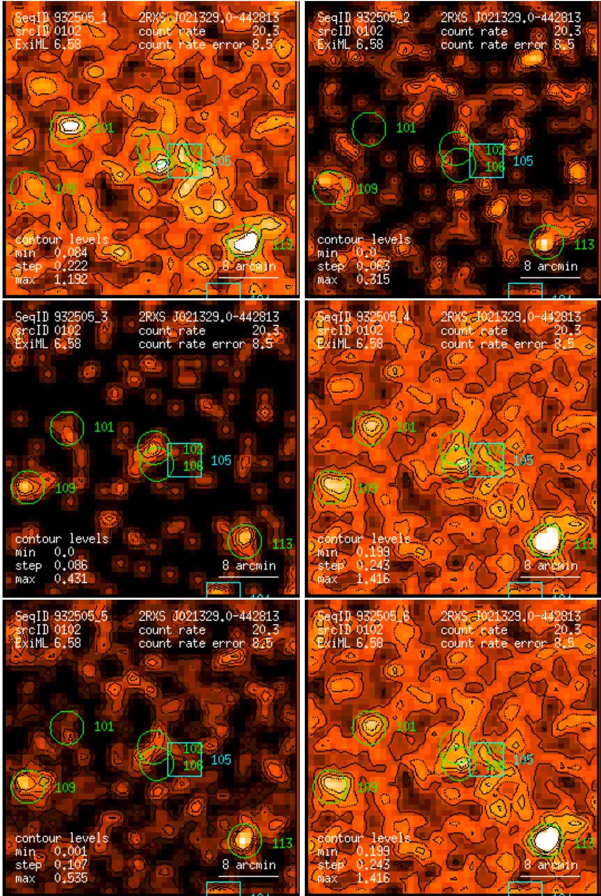
Figure 102: RASS 932505: detection 0102: band rate images, Gaussian filter: (1) PSPC channels 11 – 41, (2) 52 – 90, (3) 91 – 201, (4) 11 – 235, (5) 52 – 201, (6) 11 – 201. Broad band rates in counts/ks. Band rate contour levels in counts/ks/arcmin 2 .
