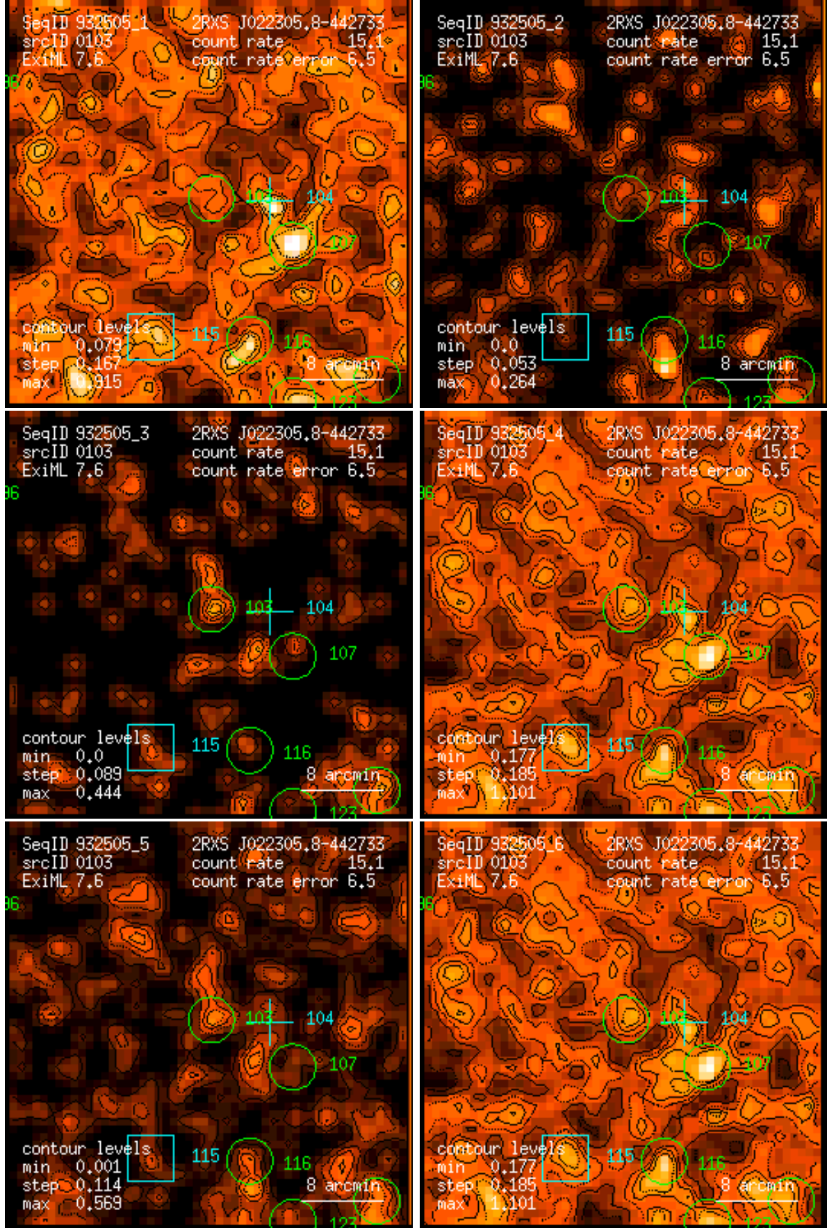
Figure 103: RASS 932505: detection 0103: band rate images, Gaussian filter: (1) PSPC channels 11 – 41, (2) 52 – 90, (3) 91 – 201, (4) 11 – 235, (5) 52 – 201, (6) 11 – 201. Broad band rates in counts/ks. Band rate contour levels in counts/ks/arcmin 2 .
