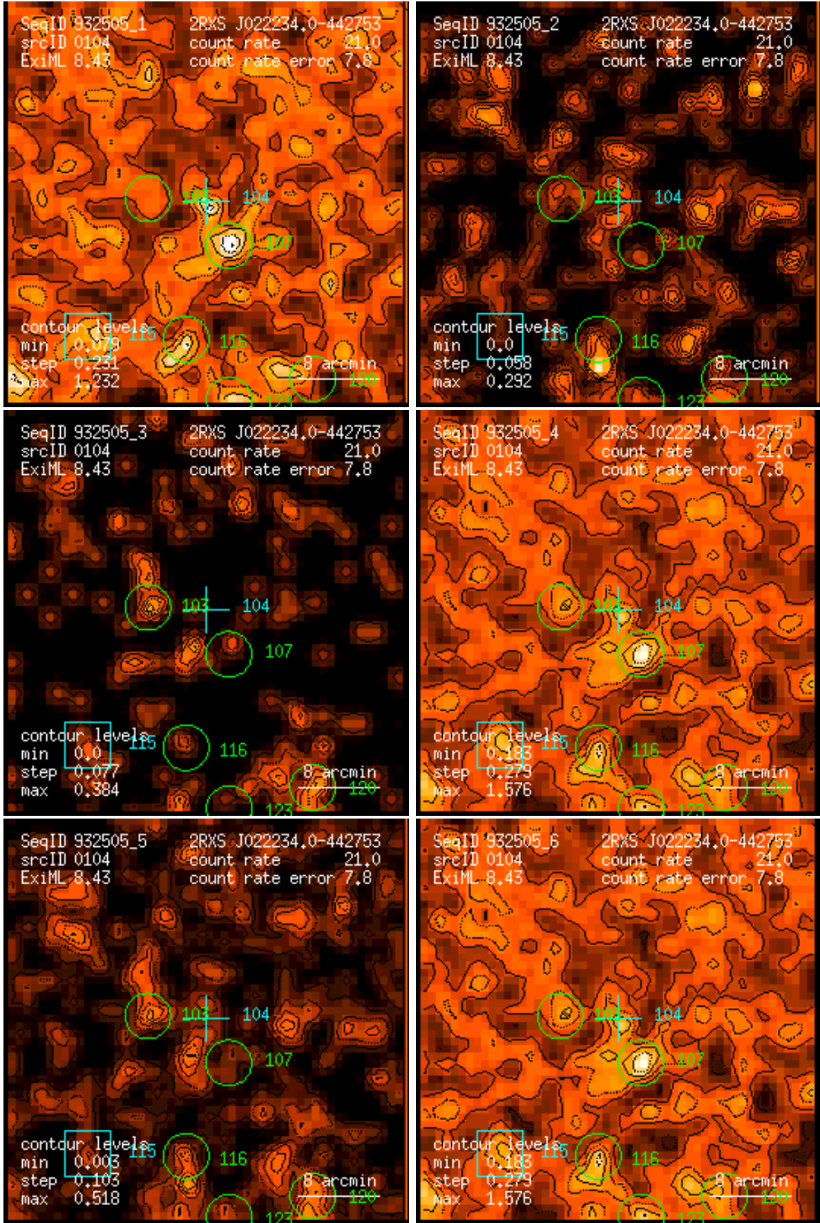
Figure 104: RASS 932505: detection 0104: band rate images, Gaussian filter: (1) PSPC channels 11 – 41, (2) 52 – 90, (3) 91 – 201, (4) 11 – 235, (5) 52 – 201, (6) 11 – 201. Broad band rates in counts/ks. Band rate contour levels in counts/ks/arcmin 2 .
