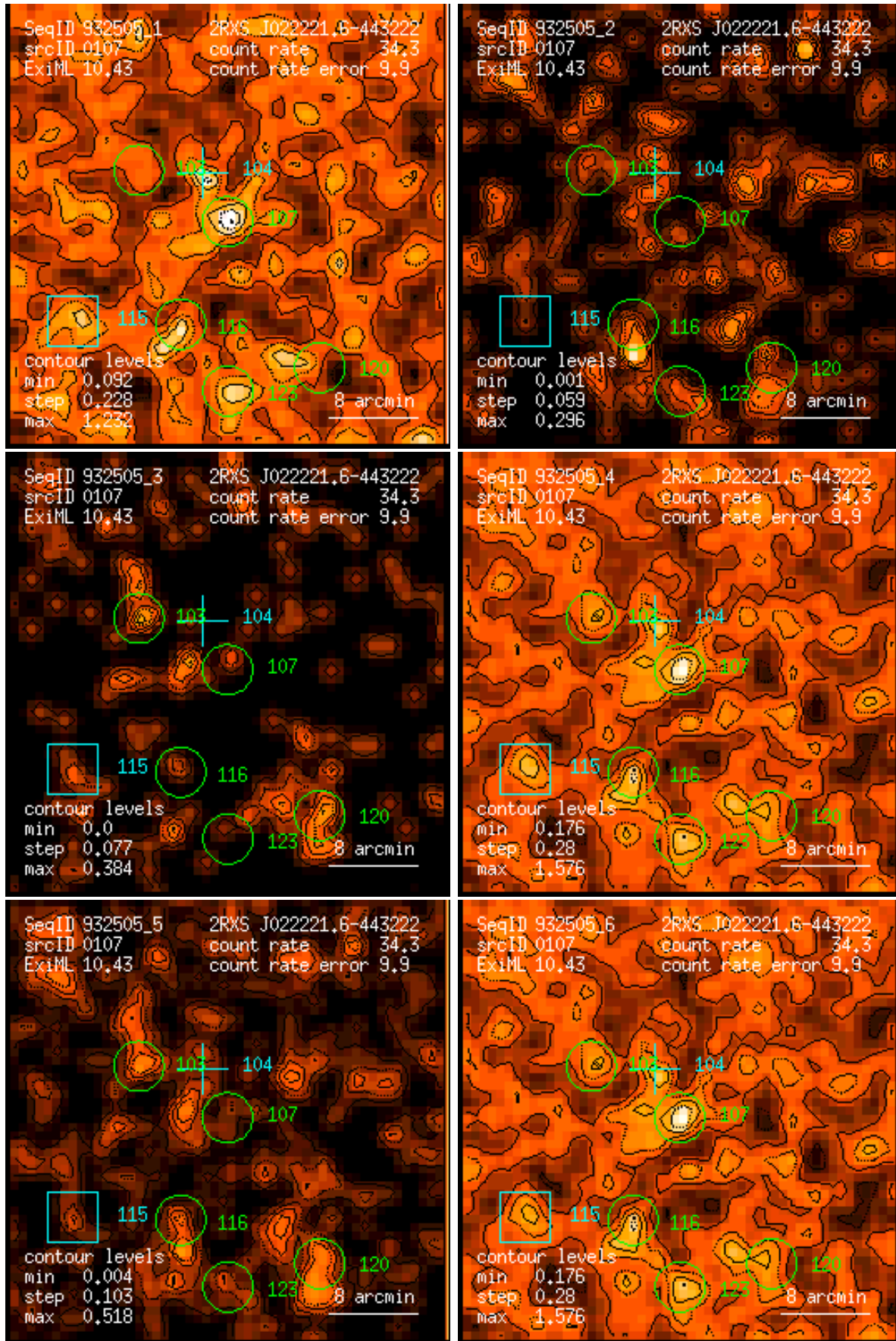
Figure 107: RASS 932505: detection 0107: band rate images, Gaussian filter: (1) PSPC channels 11 – 41, (2) 52 – 90, (3) 91 – 201, (4) 11 – 235, (5) 52 – 201, (6) 11 – 201. Broad band rates in counts/ks. Band rate contour levels in counts/ks/arcmin 2 .
