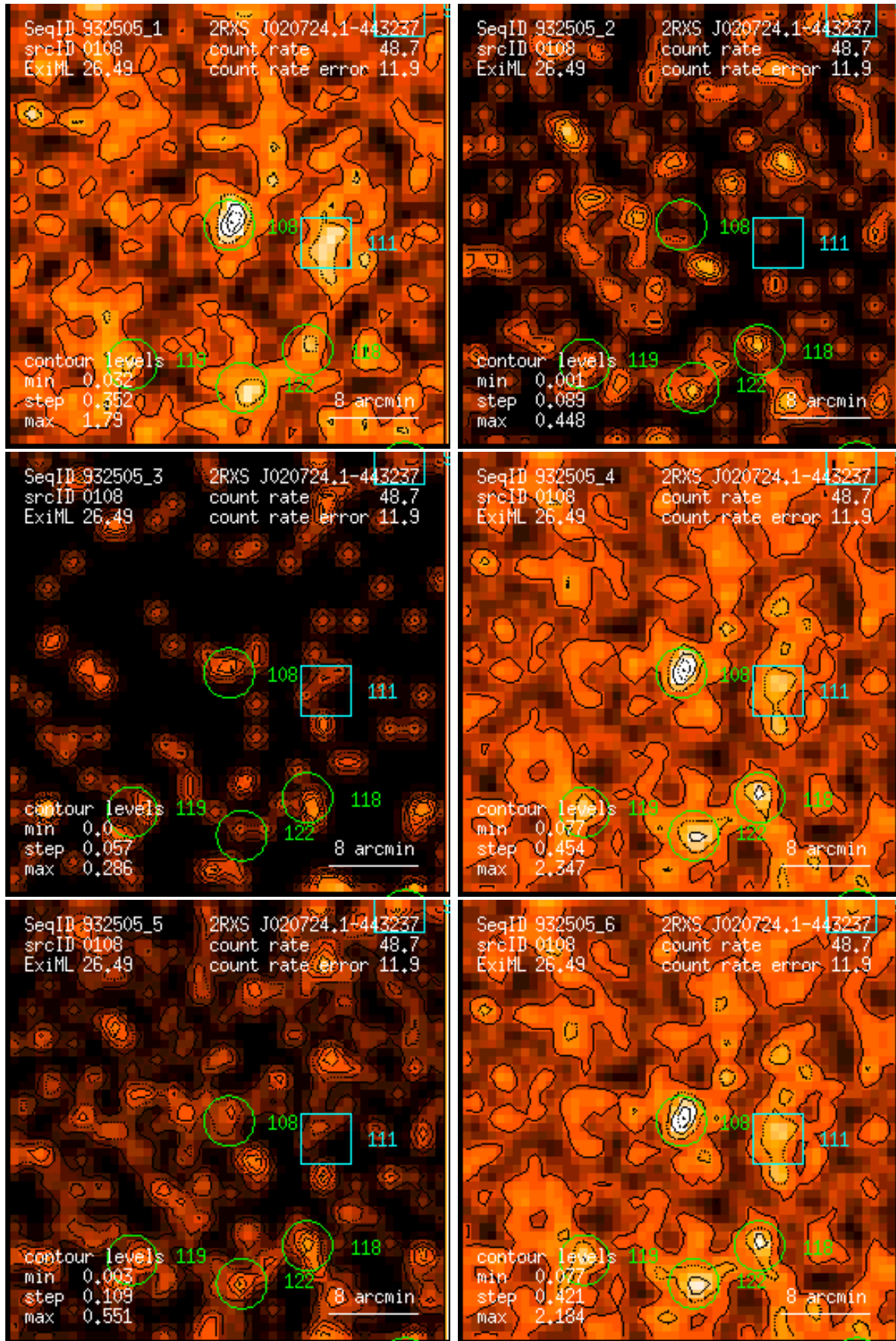
Figure 108: RASS 932505: detection 0108: band rate images, Gaussian filter: (1) PSPC channels 11 – 41, (2) 52 – 90, (3) 91 – 201, (4) 11 – 235, (5) 52 – 201, (6) 11 – 201. Broad band rates in counts/ks. Band rate contour levels in counts/ks/arcmin 2 .
