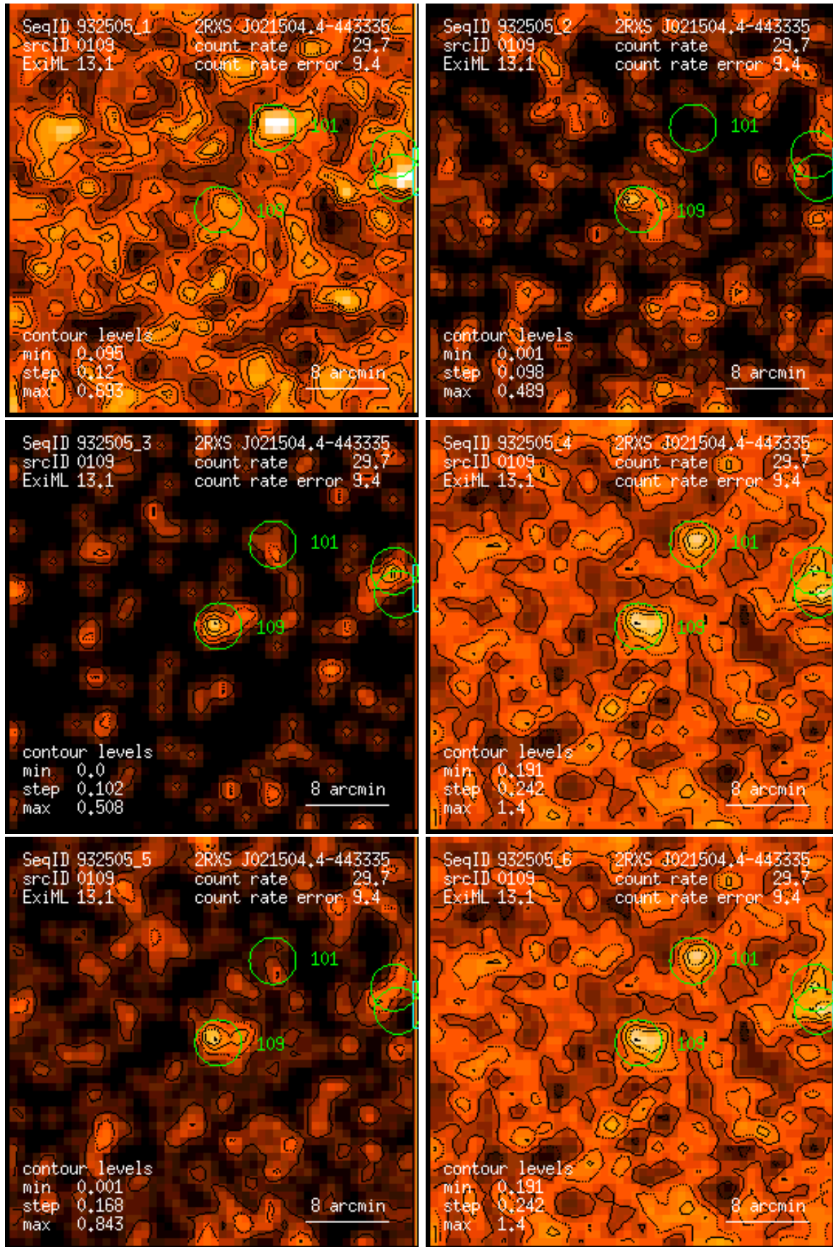
Figure 109: RASS 932505: detection 0109: band rate images, Gaussian filter: (1) PSPC channels 11 – 41, (2) 52 – 90, (3) 91 – 201, (4) 11 – 235, (5) 52 – 201, (6) 11 – 201. Broad band rates in counts/ks. Band rate contour levels in counts/ks/arcmin 2 .
