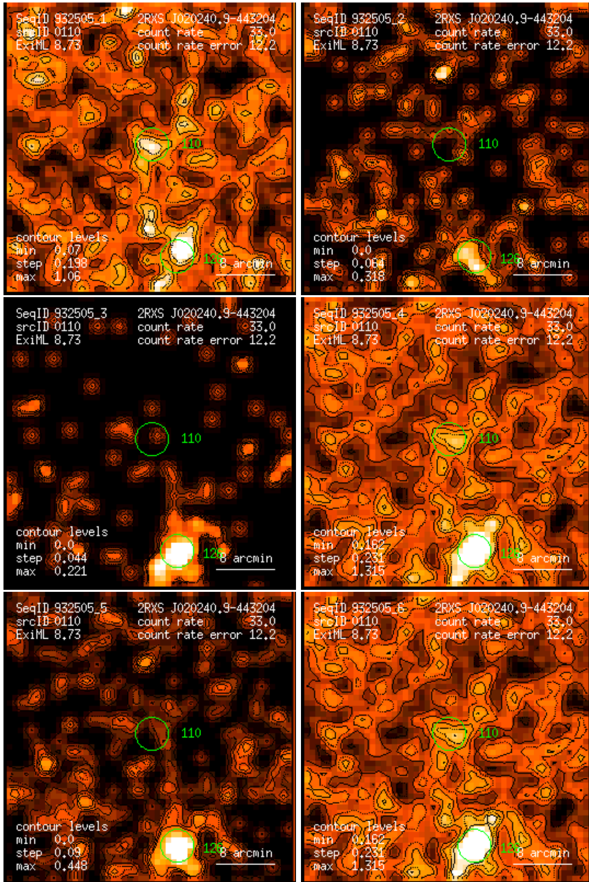
Figure 110: RASS 932505: detection 0110: band rate images, Gaussian filter: (1) PSPC channels 11 – 41, (2) 52 – 90, (3) 91 – 201, (4) 11 – 235, (5) 52 – 201, (6) 11 – 201. Broad band rates in counts/ks. Band rate contour levels in counts/ks/arcmin 2 .
