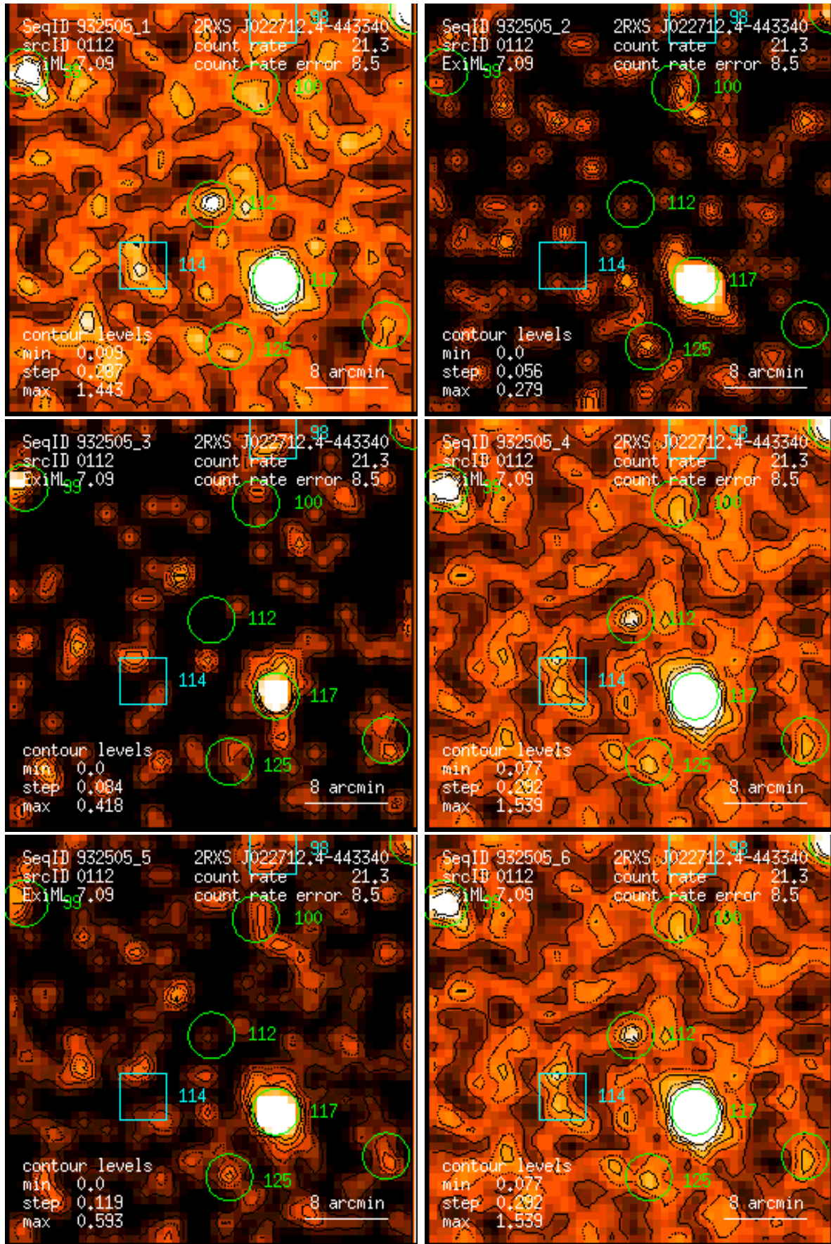
Figure 112: RASS 932505: detection 0112: band rate images, Gaussian filter: (1) PSPC channels 11 – 41, (2) 52 – 90, (3) 91 – 201, (4) 11 – 235, (5) 52 – 201, (6) 11 – 201. Broad band rates in counts/ks. Band rate contour levels in counts/ks/arcmin 2 .
