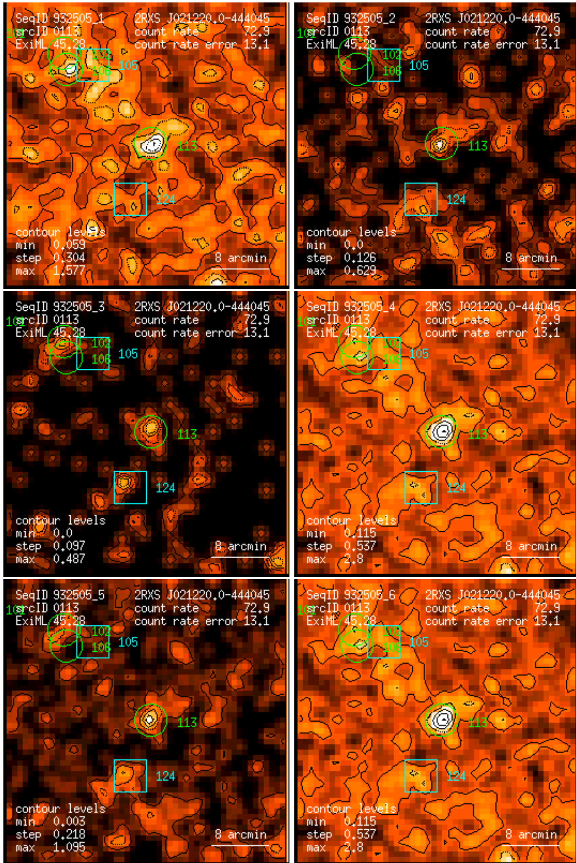
Figure 113: RASS 932505: detection 0113: band rate images, Gaussian filter: (1) PSPC channels 11 – 41, (2) 52 – 90, (3) 91 – 201, (4) 11 – 235, (5) 52 – 201, (6) 11 – 201. Broad band rates in counts/ks. Band rate contour levels in counts/ks/arcmin 2 .
