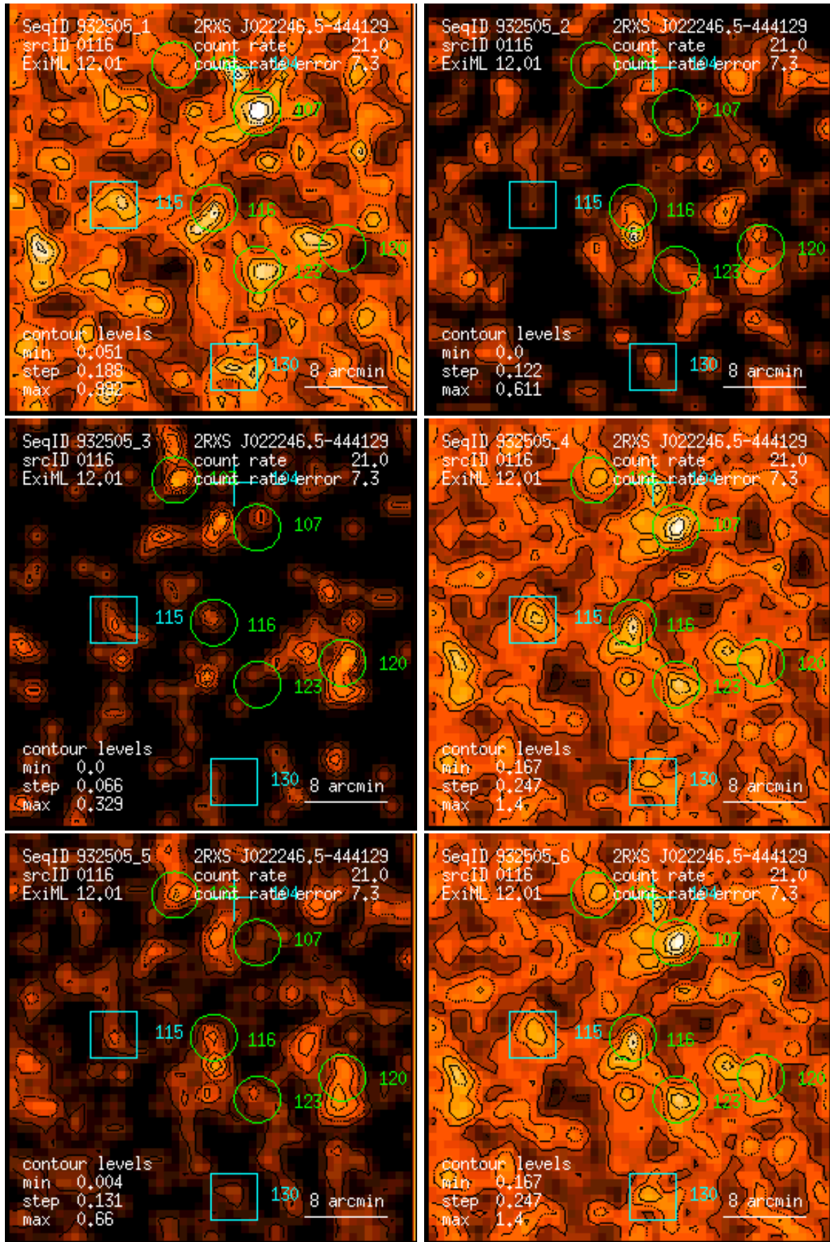
Figure 116: RASS 932505: detection 0116: band rate images, Gaussian filter: (1) PSPC channels 11 – 41, (2) 52 – 90, (3) 91 – 201, (4) 11 – 235, (5) 52 – 201, (6) 11 – 201. Broad band rates in counts/ks. Band rate contour levels in counts/ks/arcmin 2 .
