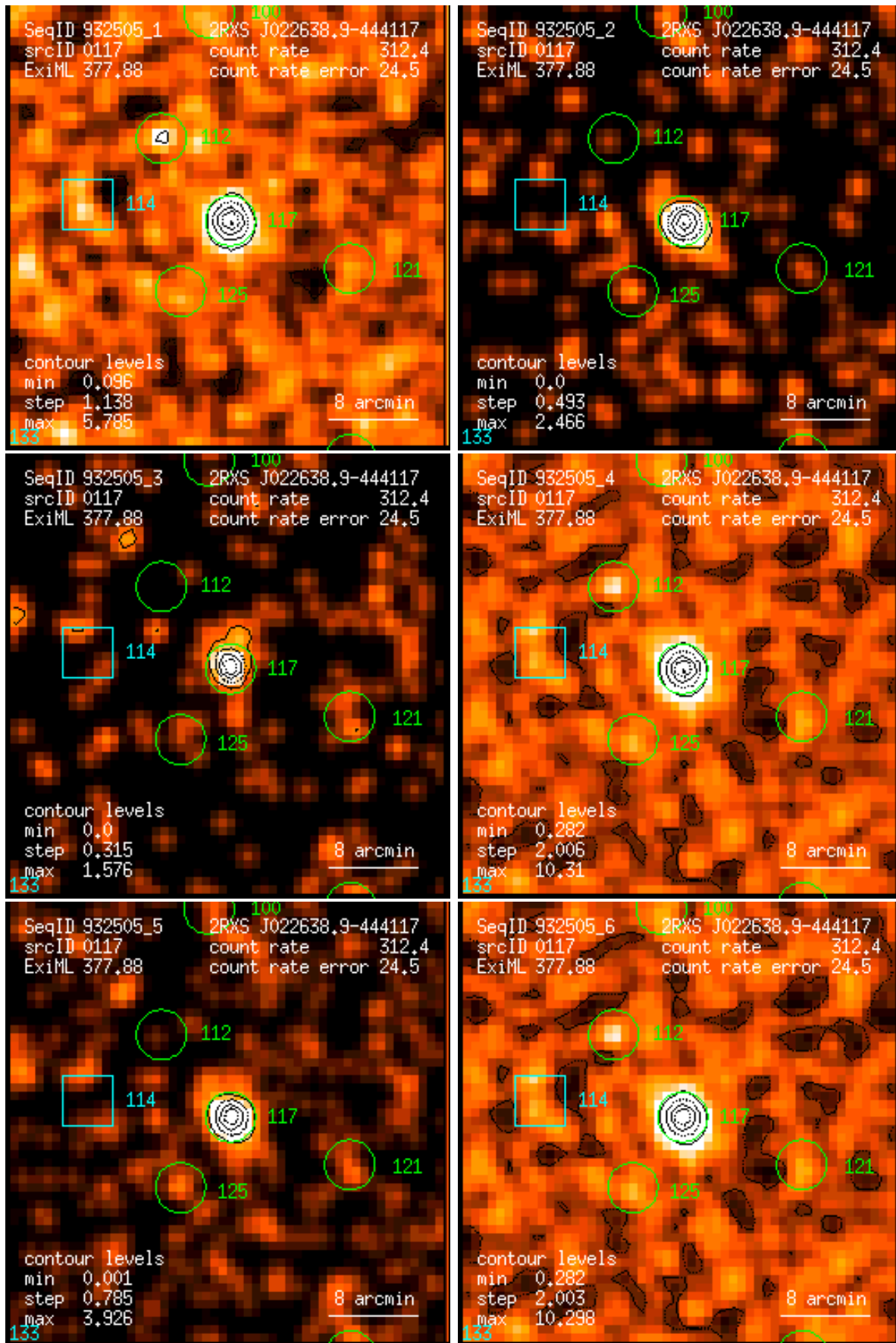
Figure 117: RASS 932505: detection 0117: band rate images, Gaussian filter: (1) PSPC channels 11 – 41, (2) 52 – 90, (3) 91 – 201, (4) 11 – 235, (5) 52 – 201, (6) 11 – 201. Broad band rates in counts/ks. Band rate contour levels in counts/ks/arcmin 2 .
