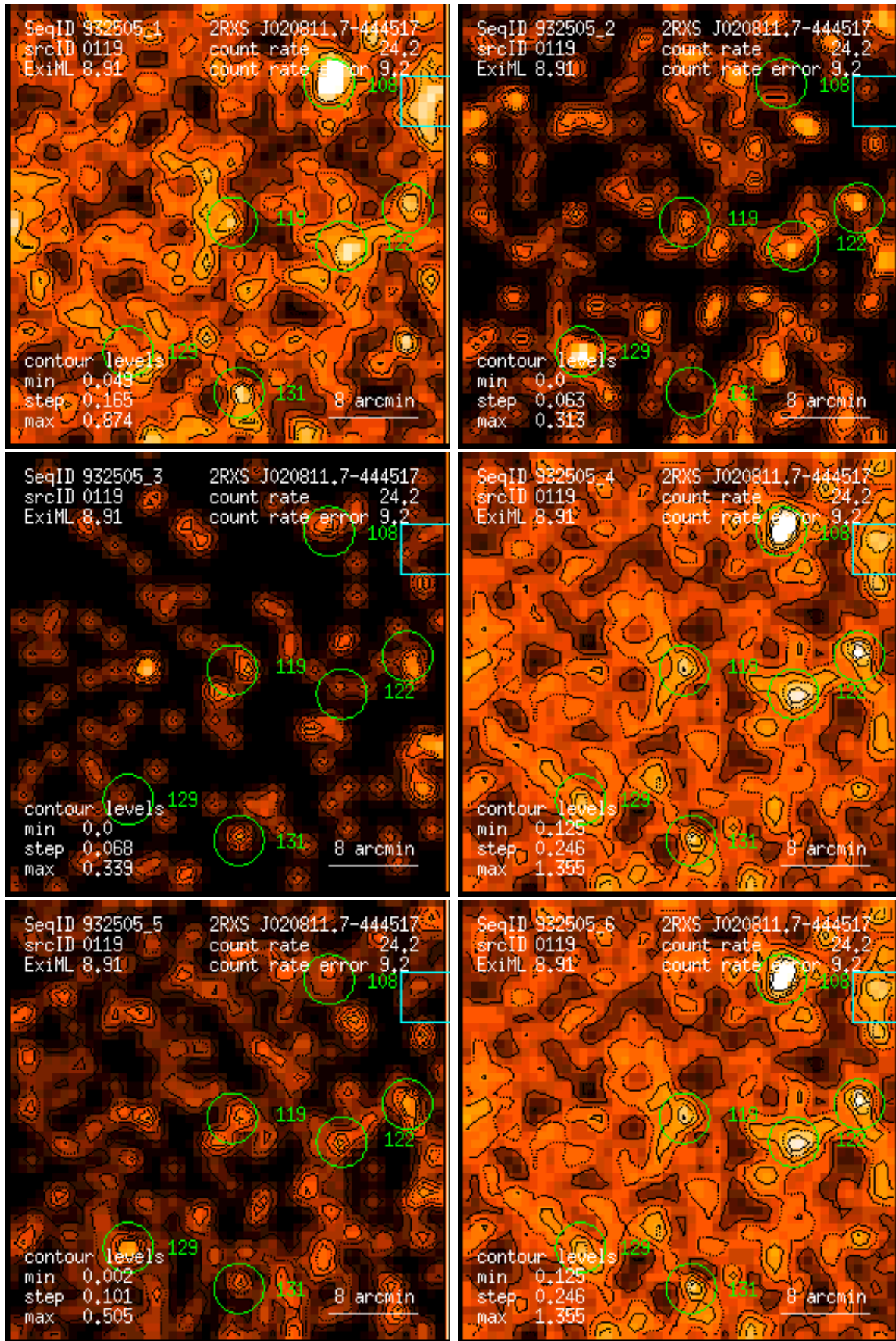
Figure 119: RASS 932505: detection 0119: band rate images, Gaussian filter: (1) PSPC channels 11 – 41, (2) 52 – 90, (3) 91 – 201, (4) 11 – 235, (5) 52 – 201, (6) 11 – 201. Broad band rates in counts/ks. Band rate contour levels in counts/ks/arcmin 2 .
