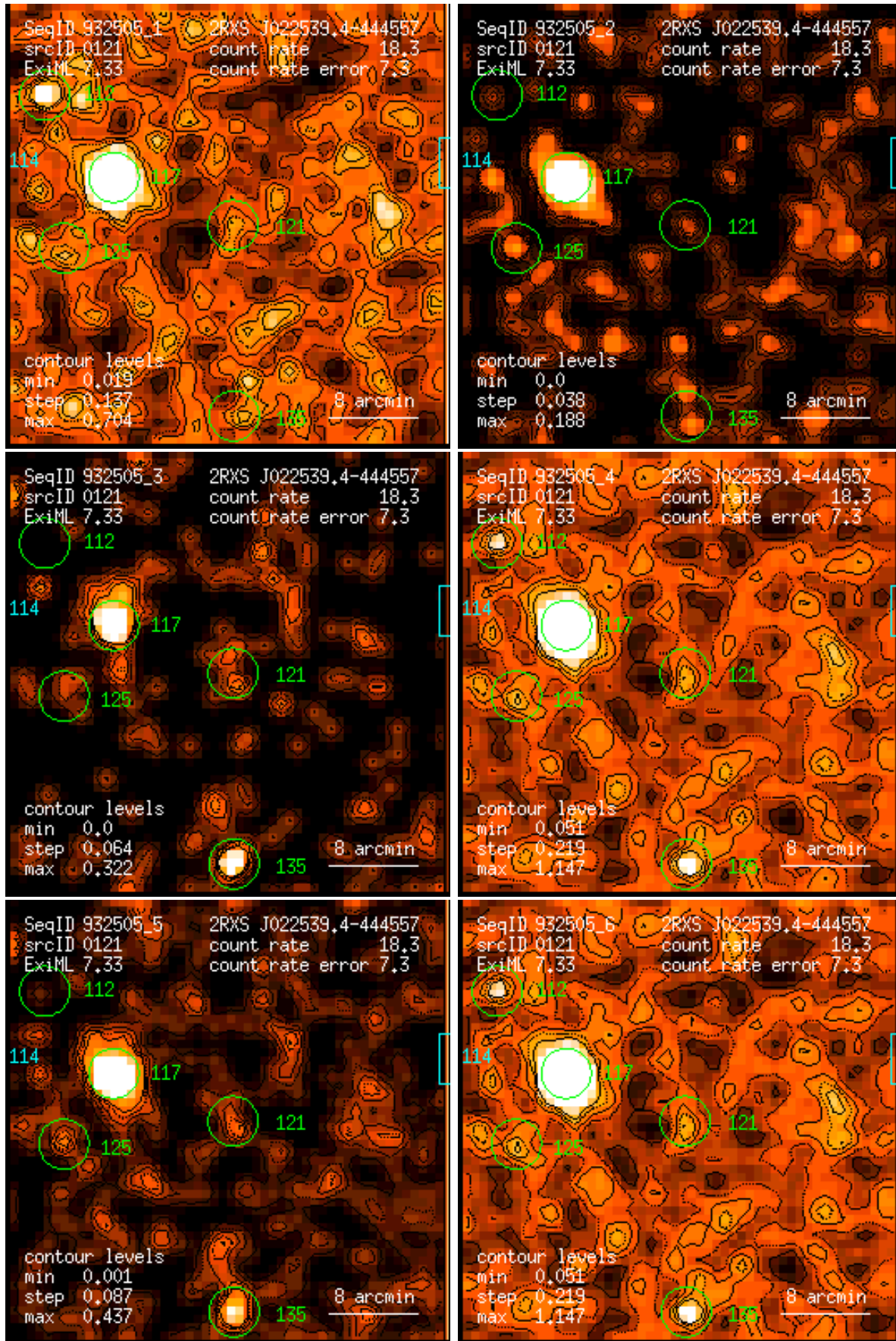
Figure 121: RASS 932505: detection 0121: band rate images, Gaussian filter: (1) PSPC channels 11 – 41, (2) 52 – 90, (3) 91 – 201, (4) 11 – 235, (5) 52 – 201, (6) 11 – 201. Broad band rates in counts/ks. Band rate contour levels in counts/ks/arcmin 2 .
