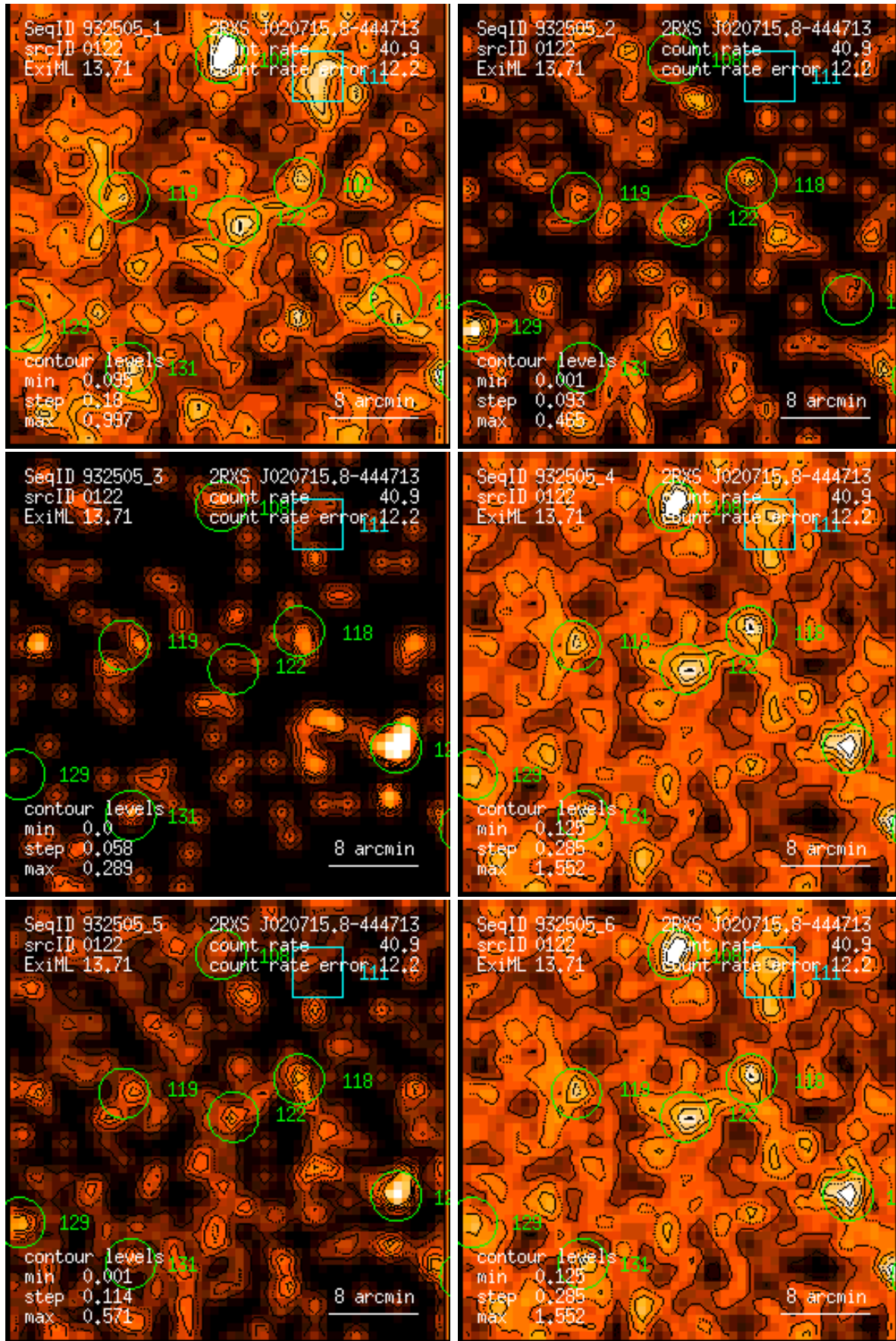
Figure 122: RASS 932505: detection 0122: band rate images, Gaussian filter: (1) PSPC channels 11 – 41, (2) 52 – 90, (3) 91 – 201, (4) 11 – 235, (5) 52 – 201, (6) 11 – 201. Broad band rates in counts/ks. Band rate contour levels in counts/ks/arcmin 2 .
