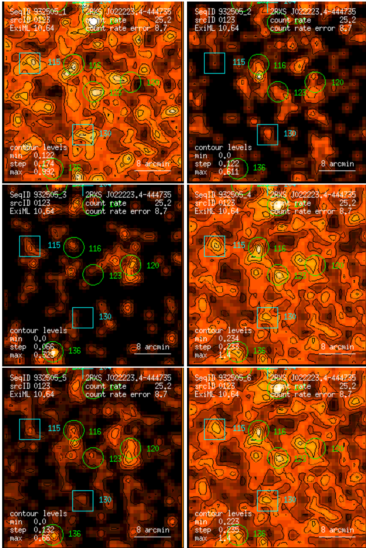
Figure 123: RASS 932505: detection 0123: band rate images, Gaussian filter: (1) PSPC channels 11 – 41, (2) 52 – 90, (3) 91 – 201, (4) 11 – 235, (5) 52 – 201, (6) 11 – 201. Broad band rates in counts/ks. Band rate contour levels in counts/ks/arcmin 2 .
